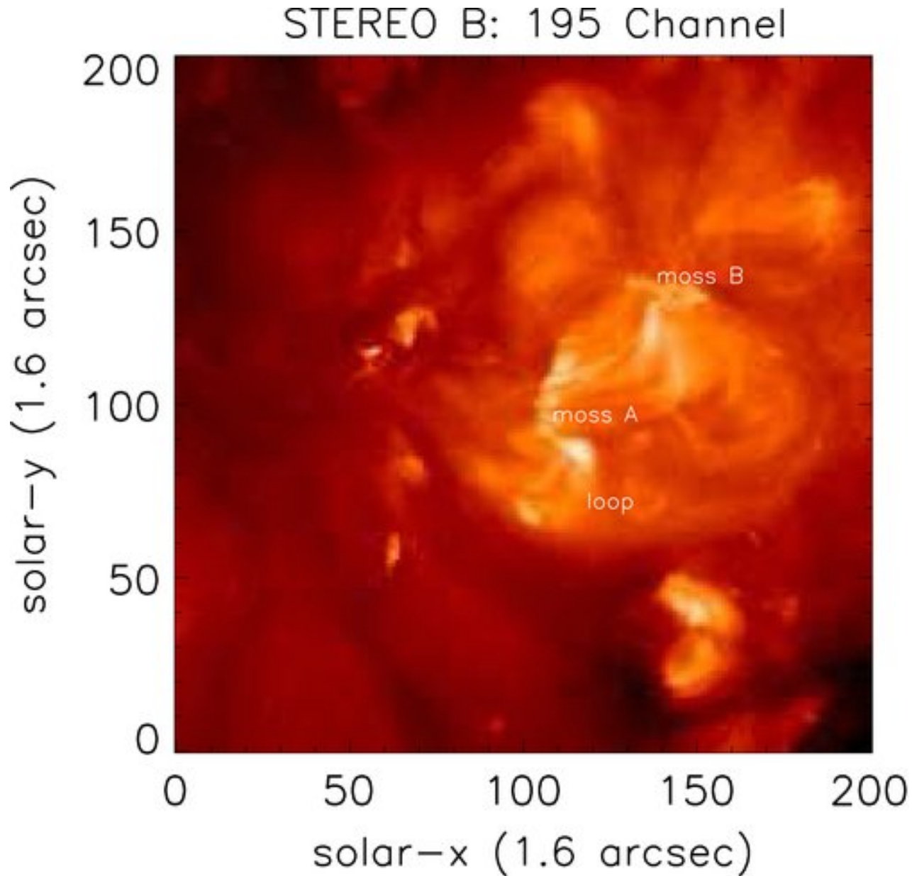
Figure 5. from Estimating the Chromospheric Absorption of Transition Region Moss Emission De PONTIEU ET AL. 2009 ApJ 702 1016 doi:10.1088/0004-637X/702/2/1016 https://dx.doi.org/10.1088/0004-637X/702/2/1016 © 2009. The American Astronomical Society. All rights reserved.
