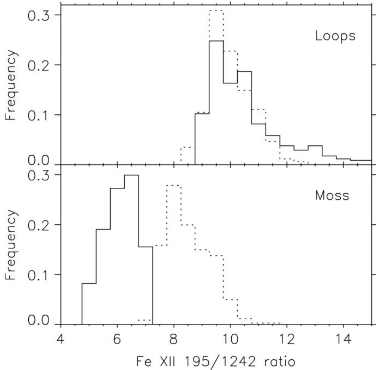
Figure 2. from Estimating the Chromospheric Absorption of Transition Region Moss Emission De PONTIEU ET AL. 2009 ApJ 702 1016 doi:10.1088/0004-637X/702/2/1016 https://dx.doi.org/10.1088/0004-637X/702/2/1016 © 2009. The American Astronomical Society. All rights reserved.
