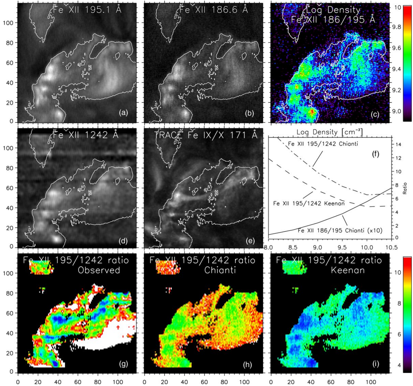
Figure 1. from Estimating the Chromospheric Absorption of Transition Region Moss Emission De PONTIEU ET AL. 2009 ApJ 702 1016 doi:10.1088/0004-637X/702/2/1016 https://dx.doi.org/10.1088/0004-637X/702/2/1016 © 2009. The American Astronomical Society. All rights reserved.
