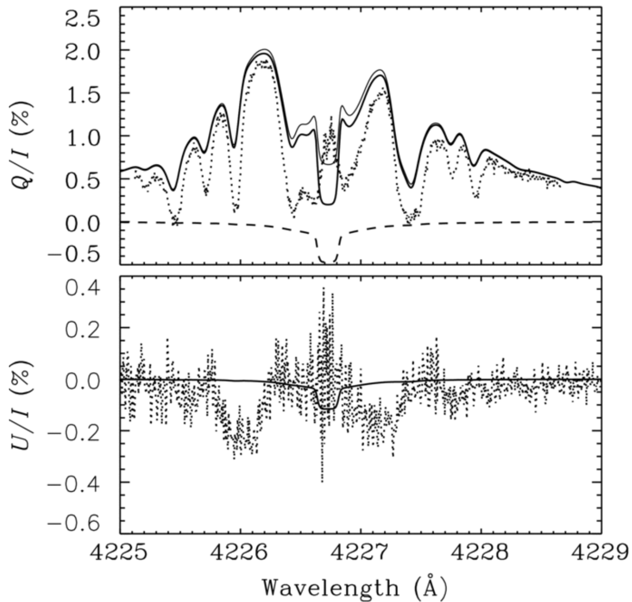
Figure 7. from Origin of Spatial Variations of Scattering Polarization in the Wings of the Ca I 4227 Å Line SAMPOORNA ET AL. 2009 ApJ 699 1650 doi:10.1088/0004-637X/699/2/1650 https://dx.doi.org/10.1088/0004-637X/699/2/1650 © 2009. The American Astronomical Society. All rights reserved.
