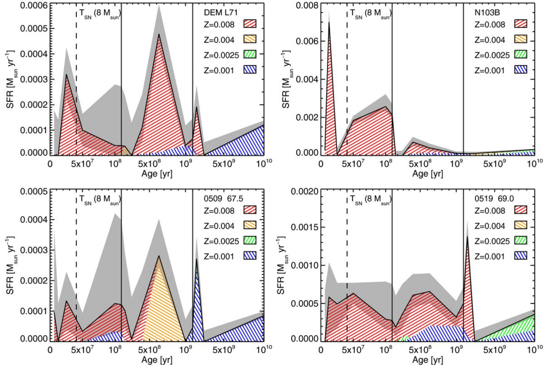
Figure 6. from The Stellar Ancestry of Supernovae in the Magellanic Clouds. I. The Most Recent Supernovae in the Large Magellanic Cloud BADENES ET AL. 2009 ApJ 700 727 doi:10.1088/0004-637X/700/1/727 https://dx.doi.org/10.1088/0004-637X/700/1/727
