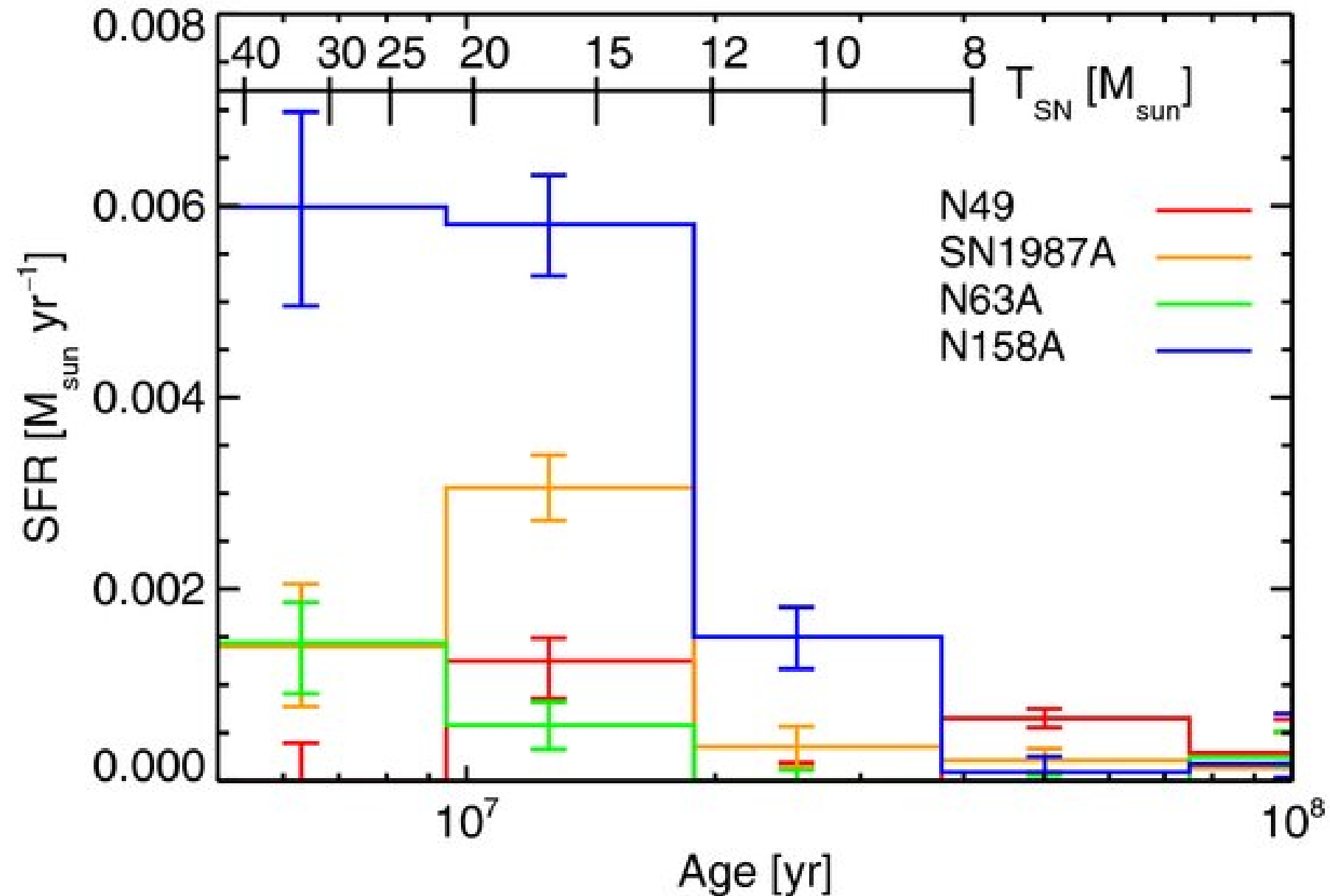
Figure 5. from The Stellar Ancestry of Supernovae in the Magellanic Clouds. I. The Most Recent Supernovae in the Large Magellanic Cloud BADENES ET AL. 2009 ApJ 700 727 doi:10.1088/0004-637X/700/1/727 https://dx.doi.org/10.1088/0004-637X/700/1/727 © 2009. The American Astronomical Society. All rights reserved.
