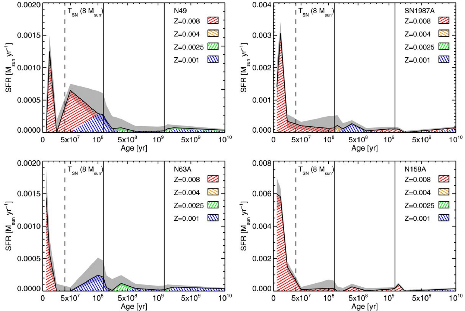
Figure 4. from The Stellar Ancestry of Supernovae in the Magellanic Clouds. I. The Most Recent Supernovae in the Large Magellanic Cloud BADENES ET AL. 2009 ApJ 700 727 doi:10.1088/0004-637X/700/1/727 https://dx.doi.org/10.1088/0004-637X/700/1/727
