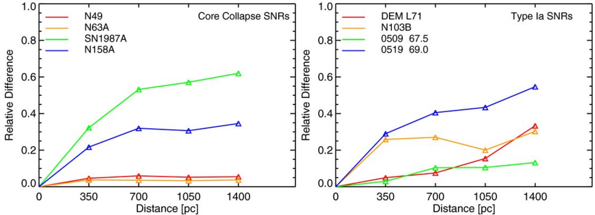
Figure 3. from The Stellar Ancestry of Supernovae in the Magellanic Clouds. I. The Most Recent Supernovae in the Large Magellanic Cloud BADENES ET AL. 2009 ApJ 700 727 doi:10.1088/0004-637X/700/1/727 https://dx.doi.org/10.1088/0004-637X/700/1/727 © 2009. The American Astronomical Society. All rights reserved.
