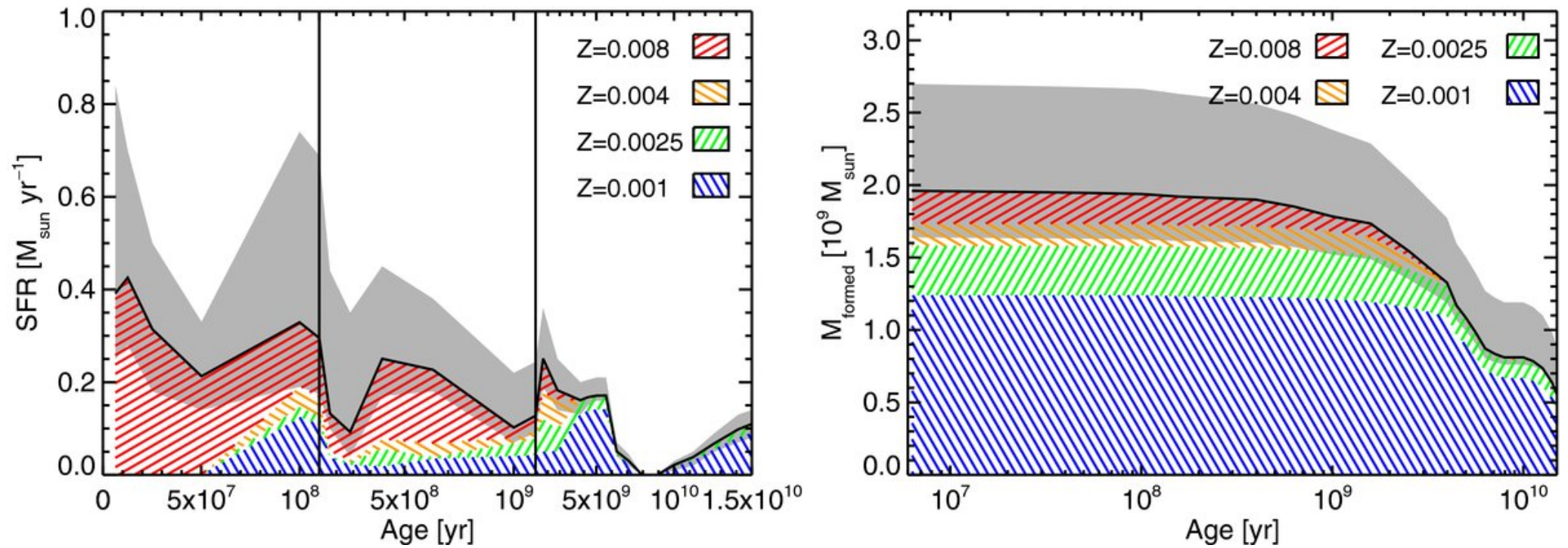
Figure 2. from The Stellar Ancestry of Supernovae in the Magellanic Clouds. I. The Most Recent Supernovae in the Large Magellanic Cloud BADENES ET AL. 2009 ApJ 700 727 doi:10.1088/0004-637X/700/1/727 https://dx.doi.org/10.1088/0004-637X/700/1/727 © 2009. The American Astronomical Society. All rights reserved.
