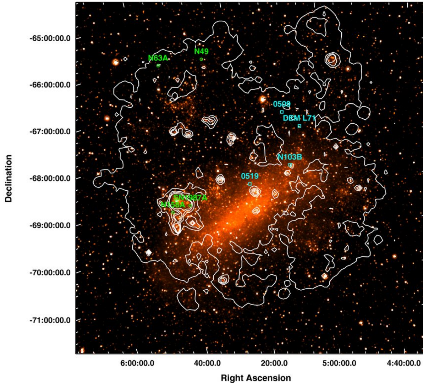
Figure 1. from The Stellar Ancestry of Supernovae in the Magellanic Clouds. I. The Most Recent Supernovae in the Large Magellanic Cloud BADENES ET AL. 2009 ApJ 700 727 doi:10.1088/0004-637X/700/1/727 https://dx.doi.org/10.1088/0004-637X/700/1/727 © 2009. The American Astronomical Society. All rights reserved.
