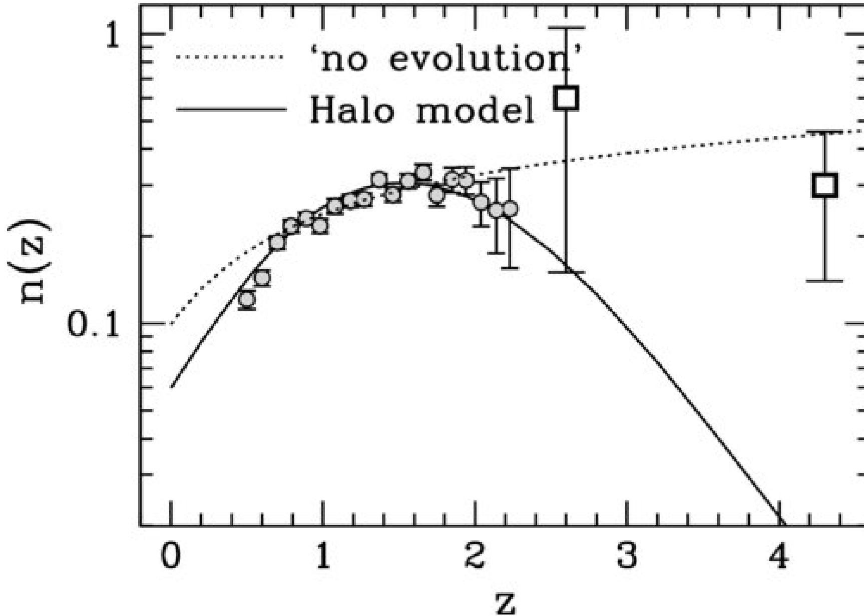
Figure 6. from On the Redshift Evolution of Mg II Absorption Systems TINKER & CHEN 2010 ApJ 709 1 doi:10.1088/0004-637X/709/1/1 https://dx.doi.org/10.1088/0004-637X/709/1/1 © 2010. The American Astronomical Society. All rights reserved.
