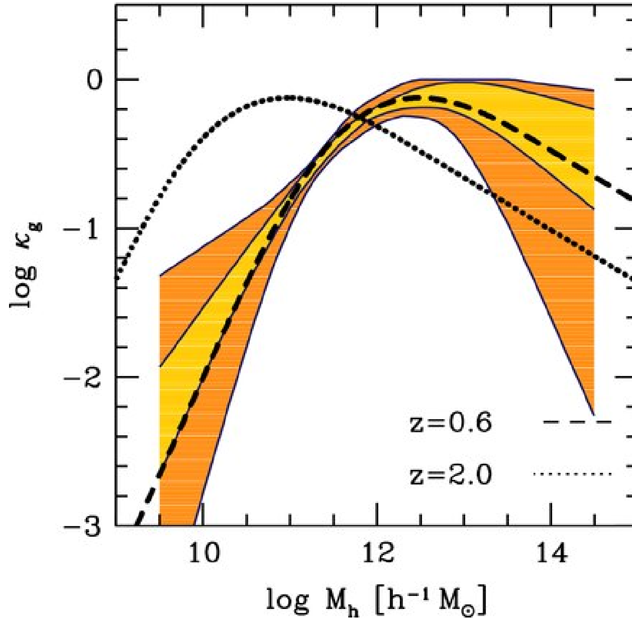
Figure 5. from On the Redshift Evolution of Mg II Absorption Systems TINKER & CHEN 2010 ApJ 709 1 doi:10.1088/0004-637X/709/1/1 https://dx.doi.org/10.1088/0004-637X/709/1/1 © 2010. The American Astronomical Society. All rights reserved.
