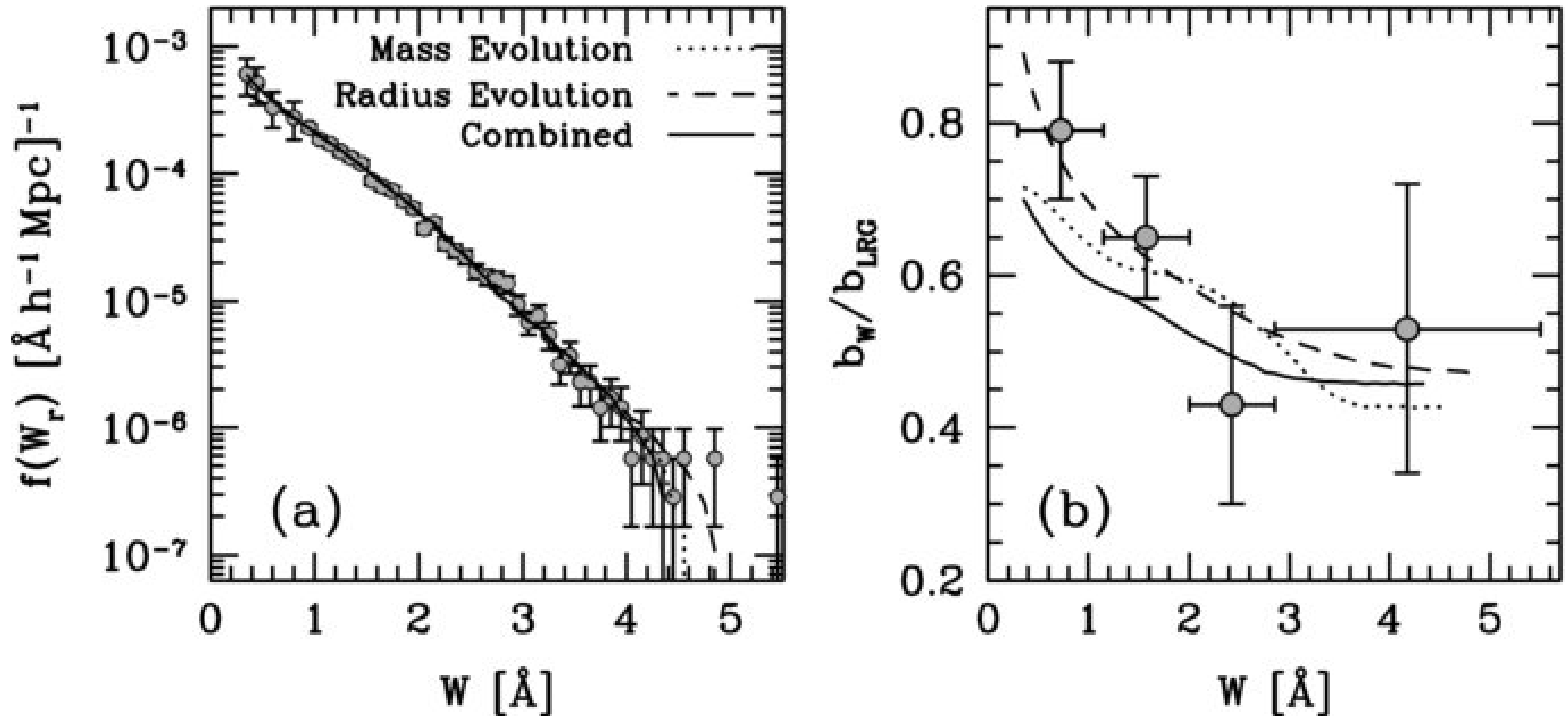
Figure 2. from On the Redshift Evolution of Mg II Absorption Systems TINKER & CHEN 2010 ApJ 709 1 doi:10.1088/0004-637X/709/1/1 https://dx.doi.org/10.1088/0004-637X/709/1/1 © 2010. The American Astronomical Society. All rights reserved.
