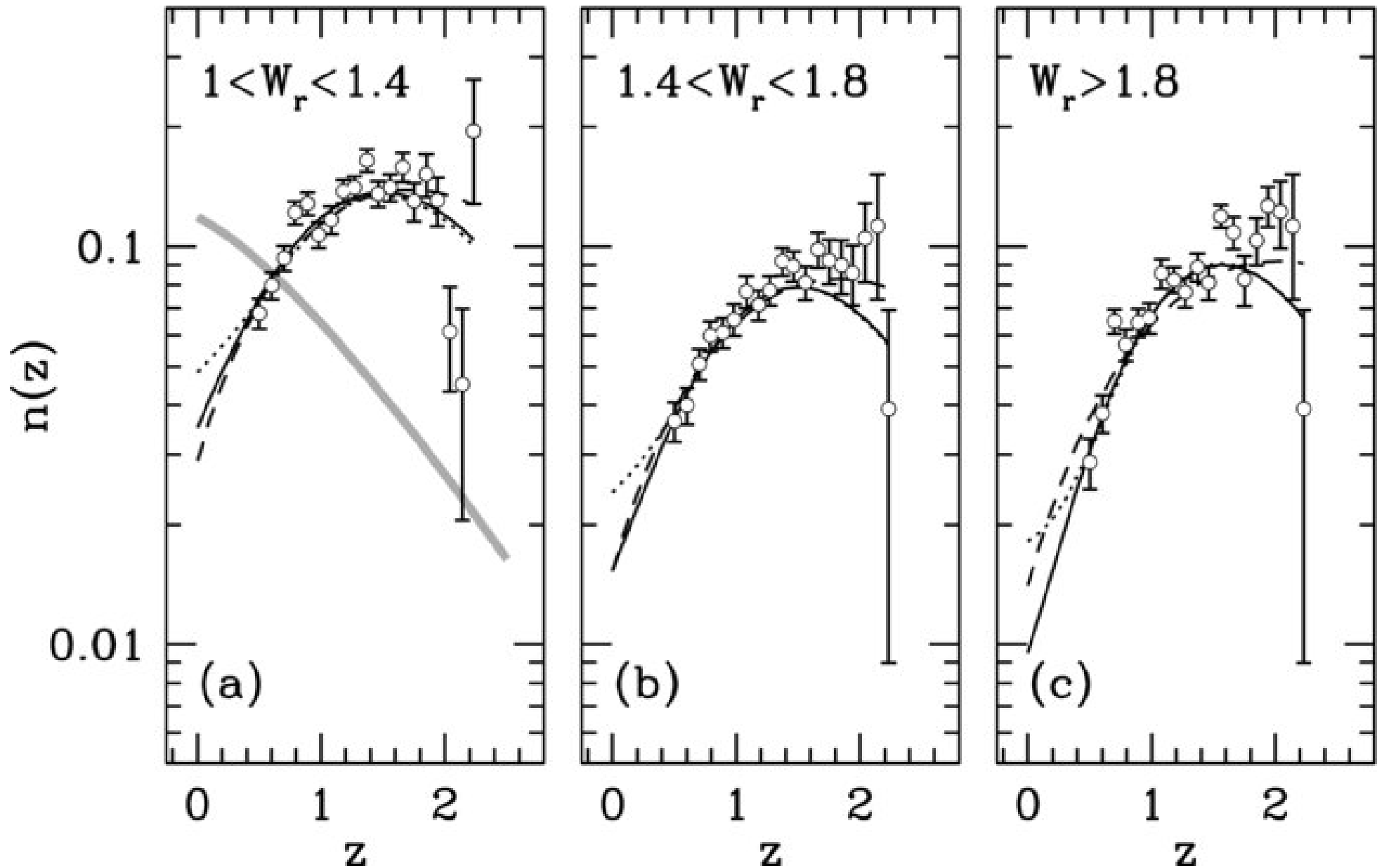
Figure 1. from On the Redshift Evolution of Mg II Absorption Systems TINKER & CHEN 2010 ApJ 709 1 doi:10.1088/0004-637X/709/1/1 https://dx.doi.org/10.1088/0004-637X/709/1/1 © 2010. The American Astronomical Society. All rights reserved.
