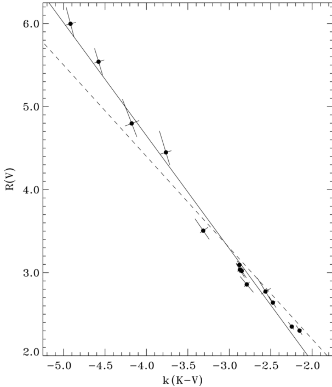
Figure 7. from An Analysis of the Shapes of Interstellar Extinction Curves. VI. The Near-IR Extinction Law FITZPATRICK & MASSA 2009 ApJ 699 1209 doi:10.1088/0004-637X/699/2/1209 https://dx.doi.org/10.1088/0004-637X/699/2/1209 © 2009. The American Astronomical Society. All rights reserved.
