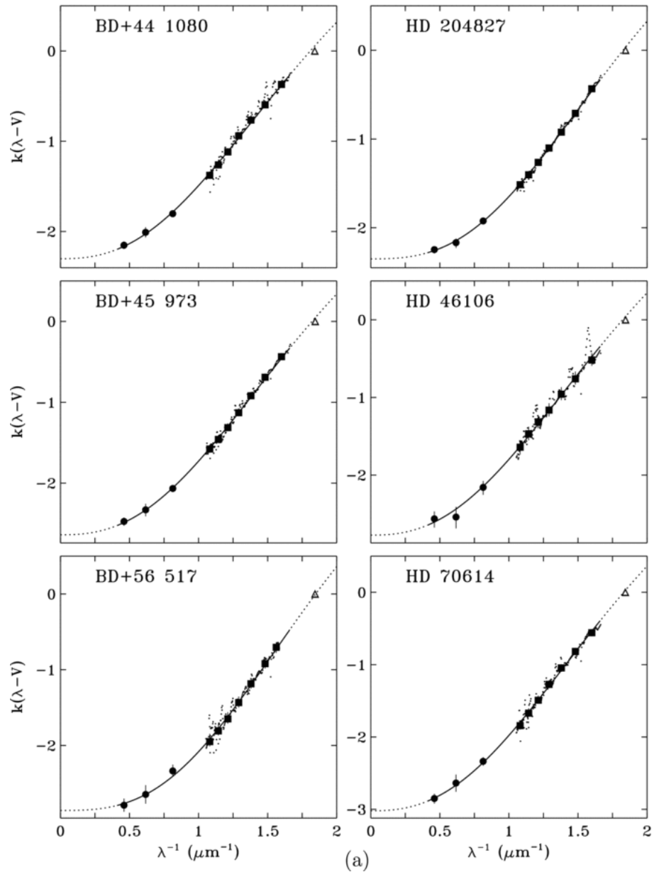
Figure 5. from An Analysis of the Shapes of Interstellar Extinction Curves. VI. The Near-IR Extinction Law FITZPATRICK & MASSA 2009 ApJ 699 1209 doi:10.1088/0004-637X/699/2/1209 https://dx.doi.org/10.1088/0004-637X/699/2/1209 © 2009. The American Astronomical Society. All rights reserved.
