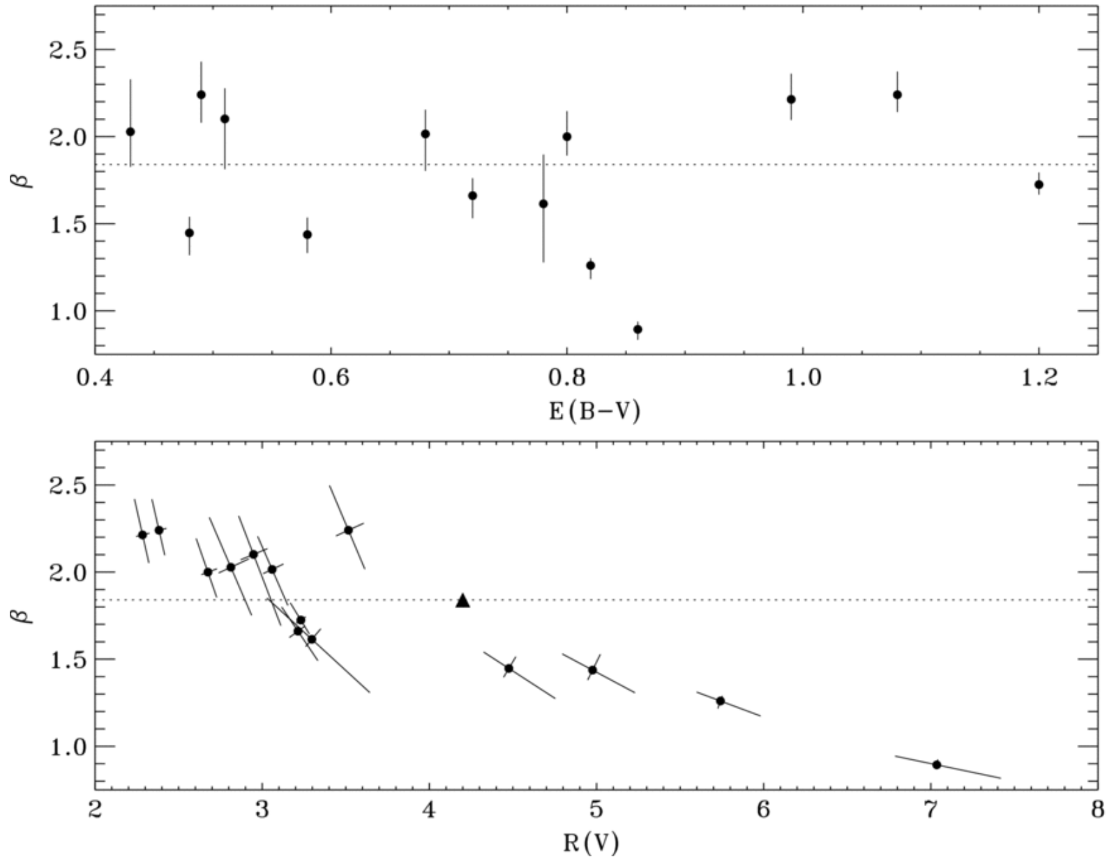
Figure 4. from An Analysis of the Shapes of Interstellar Extinction Curves. VI. The Near-IR Extinction Law FITZPATRICK & MASSA 2009 ApJ 699 1209 doi:10.1088/0004-637X/699/2/1209 https://dx.doi.org/10.1088/0004-637X/699/2/1209 © 2009. The American Astronomical Society. All rights reserved.
