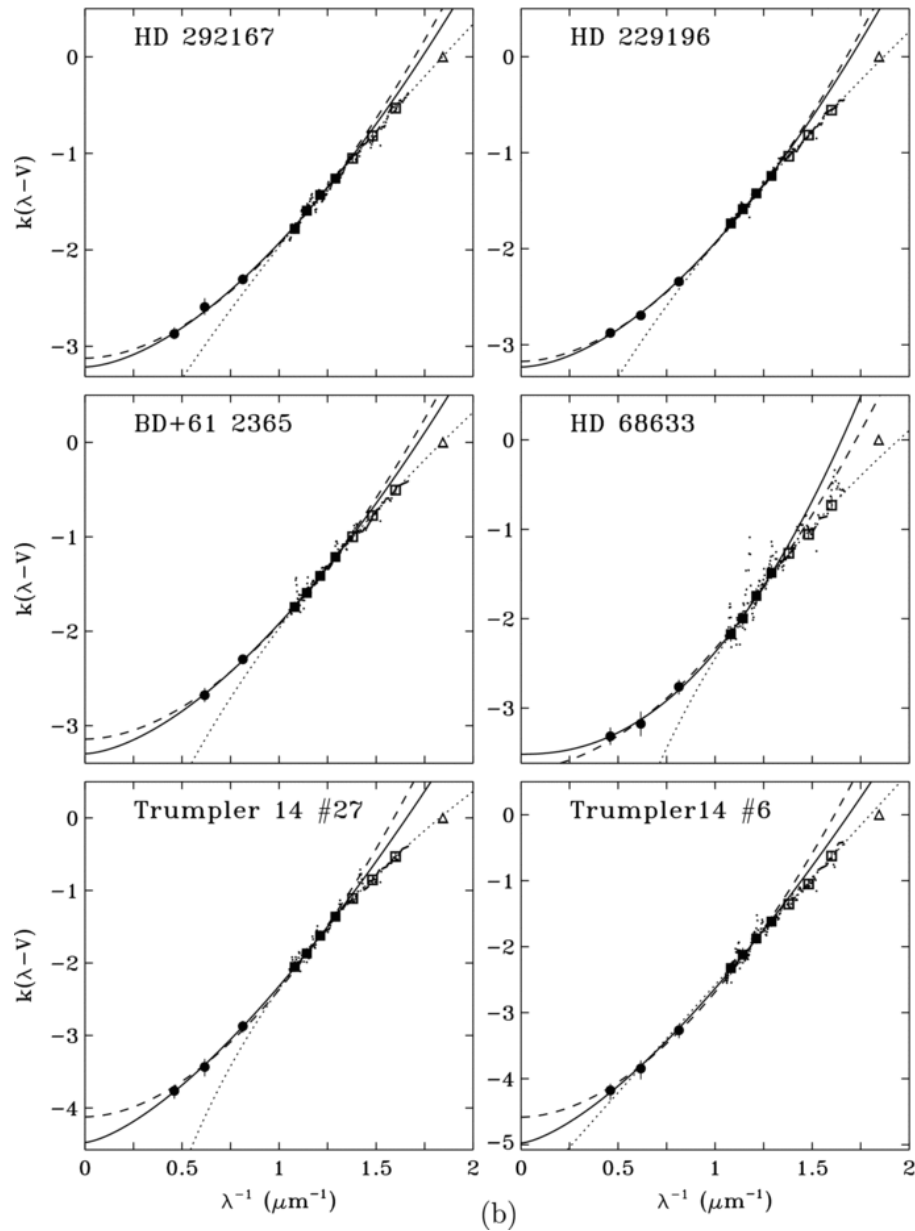
Figure 3. from An Analysis of the Shapes of Interstellar Extinction Curves. VI. The Near-IR Extinction Law FITZPATRICK & MASSA 2009 ApJ 699 1209 doi:10.1088/0004-637X/699/2/1209 https://dx.doi.org/10.1088/0004-637X/699/2/1209 © 2009. The American Astronomical Society. All rights reserved.
