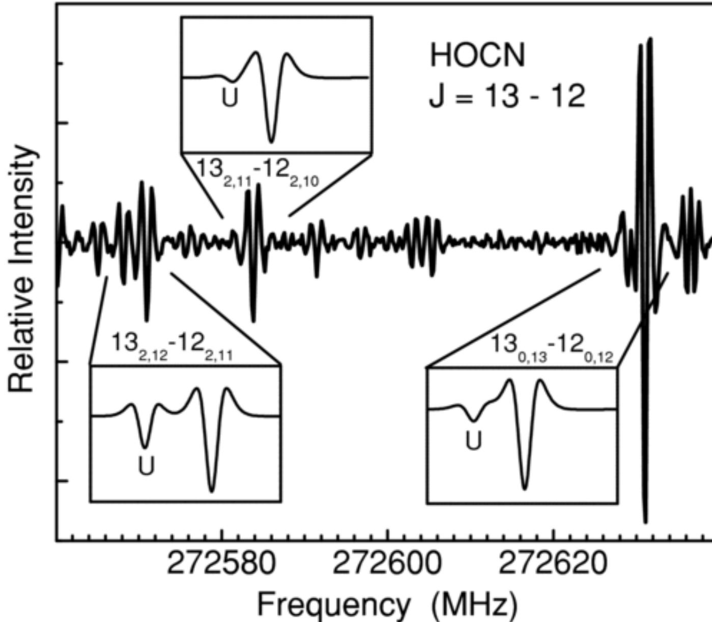
Figure 3. from Laboratory Detection of HOCN and Tentative Identification in Sgr B2 BRÜNKEN ET AL. 2009 ApJ 697 880 doi:10.1088/0004-637X/697/1/880 https://dx.doi.org/10.1088/0004-637X/697/1/880 © 2009. The American Astronomical Society. All rights reserved.
