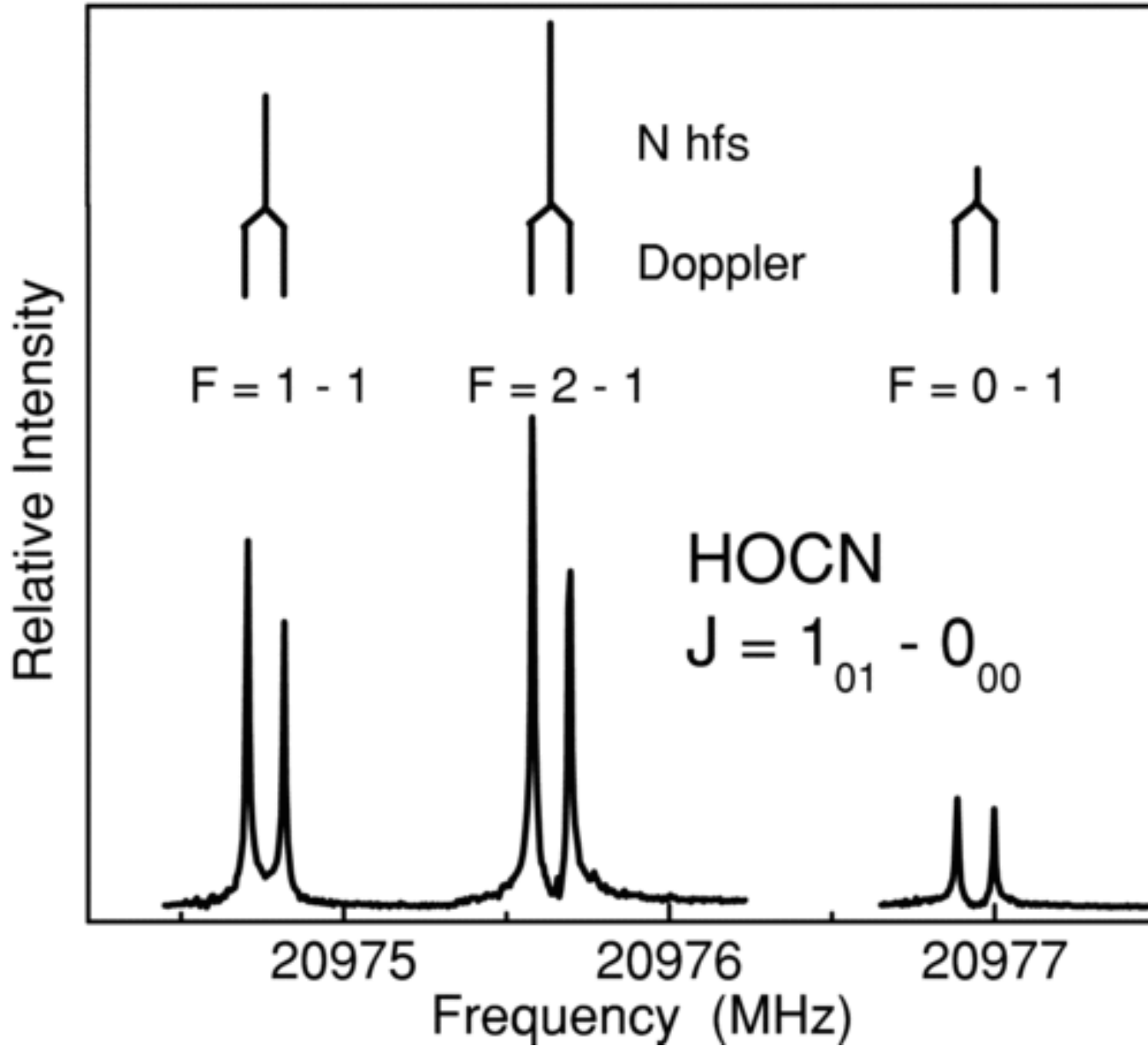
Figure 2. from Laboratory Detection of HOCN and Tentative Identification in Sgr B2 BRÜNKEN ET AL. 2009 ApJ 697 880 doi:10.1088/0004-637X/697/1/880 https://dx.doi.org/10.1088/0004-637X/697/1/880 © 2009. The American Astronomical Society. All rights reserved.
