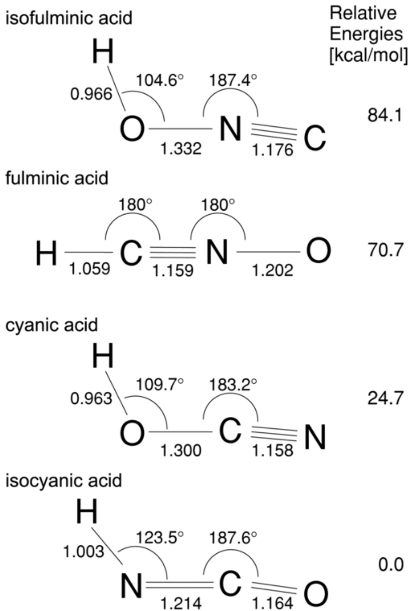
Figure 1. from Laboratory Detection of HOCN and Tentative Identification in Sgr B2 BRÜNKEN ET AL. 2009 ApJ 697 880 doi:10.1088/0004-637X/697/1/880 https://dx.doi.org/10.1088/0004-637X/697/1/880 © 2009. The American Astronomical Society. All rights reserved.
