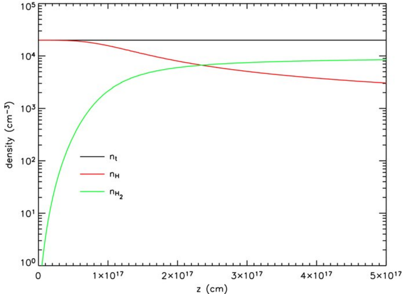
Figure 5. from Molecular Hydrogen Formation Catalyzed by Polycyclic Aromatic Hydrocarbons in the Interstellar Medium LE PAGE, SNOW & BIERBAUM 2009 ApJ 704 274 doi:10.1088/0004-637X/704/1/274 https://dx.doi.org/10.1088/0004-637X/704/1/274 © 2009. The American Astronomical Society. All rights reserved.
