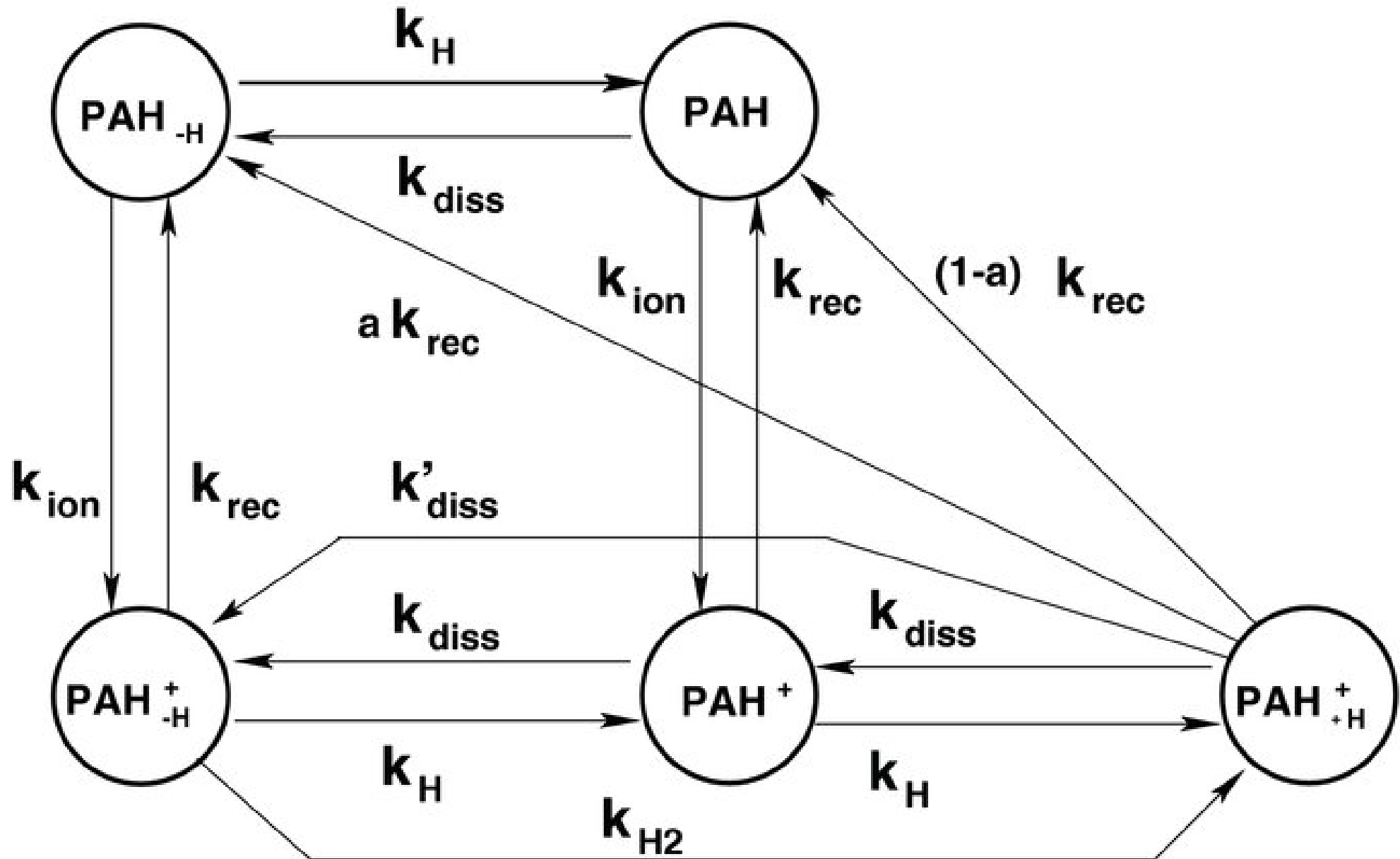
Figure 1. from Molecular Hydrogen Formation Catalyzed by Polycyclic Aromatic Hydrocarbons in the Interstellar Medium LE PAGE, SNOW & BIERBAUM 2009 ApJ 704 274 doi:10.1088/0004-637X/704/1/274 https://dx.doi.org/10.1088/0004-637X/704/1/274 © 2009. The American Astronomical Society. All rights reserved.
