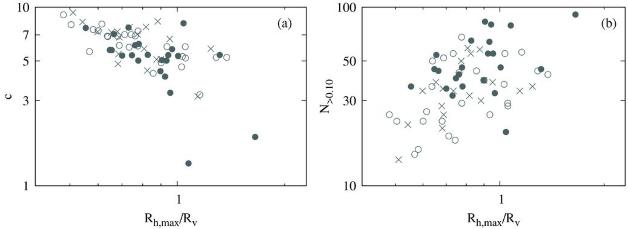
Figure 8. from Variation of the Subhalo Abundance in Dark Matter Halos ISHIYAMA, FUKUSHIGE, & MAKINO 2009 ApJ 696 2115 doi:10.1088/0004-637X/696/2/2115 https://dx.doi.org/10.1088/0004-637X/696/2/2115 © 2009. The American Astronomical Society. All rights reserved.
