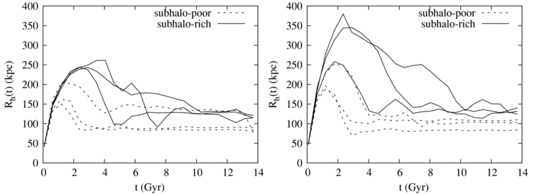
Figure 7. from Variation of the Subhalo Abundance in Dark Matter Halos ISHIYAMA, FUKUSHIGE, & MAKINO 2009 ApJ 696 2115 doi:10.1088/0004-637X/696/2/2115 https://dx.doi.org/10.1088/0004-637X/696/2/2115 © 2009. The American Astronomical Society. All rights reserved.
