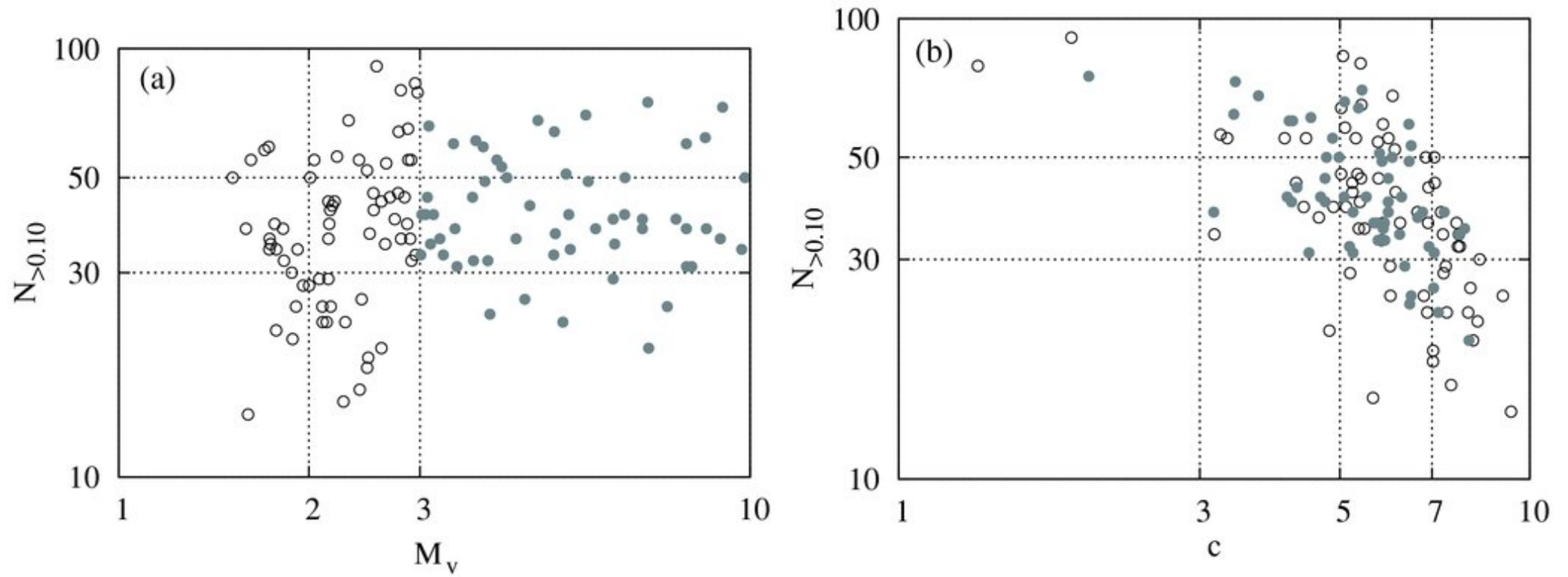
Figure 4. from Variation of the Subhalo Abundance in Dark Matter Halos ISHIYAMA, FUKUSHIGE, & MAKINO 2009 ApJ 696 2115 doi:10.1088/0004-637X/696/2/2115 https://dx.doi.org/10.1088/0004-637X/696/2/2115 © 2009. The American Astronomical Society. All rights reserved.
