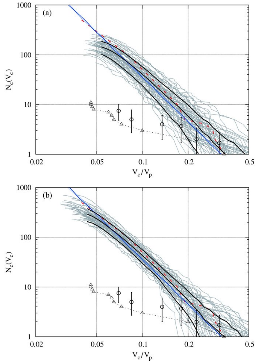
Figure 2. from Variation of the Subhalo Abundance in Dark Matter Halos ISHIYAMA, FUKUSHIGE, & MAKINO 2009 ApJ 696 2115 doi:10.1088/0004-637X/696/2/2115 https://dx.doi.org/10.1088/0004-637X/696/2/2115 © 2009. The American Astronomical Society. All rights reserved.
