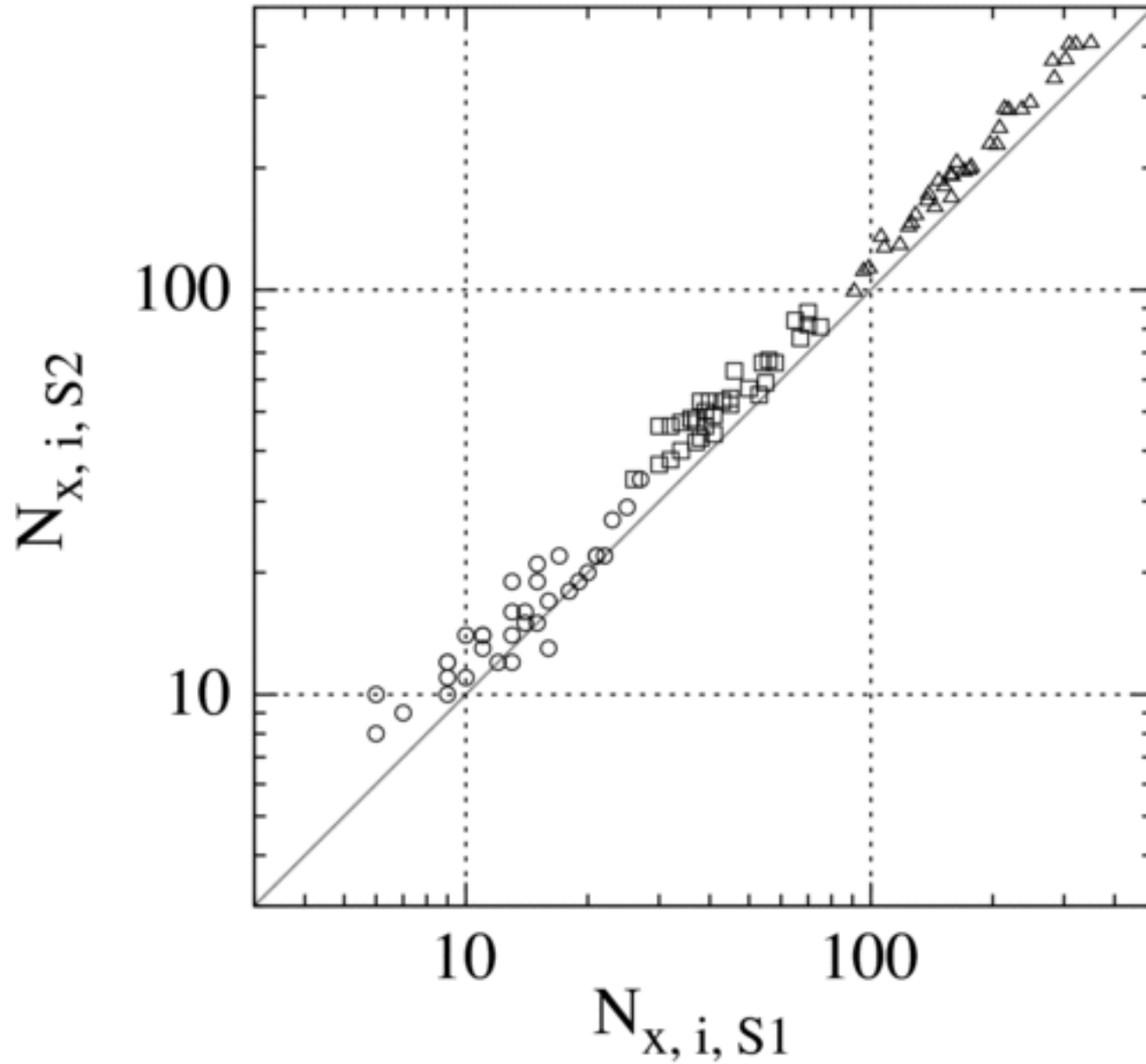
Figure 1. from Variation of the Subhalo Abundance in Dark Matter Halos ISHIYAMA, FUKUSHIGE, & MAKINO 2009 ApJ 696 2115 doi:10.1088/0004-637X/696/2/2115 https://dx.doi.org/10.1088/0004-637X/696/2/2115 © 2009. The American Astronomical Society. All rights reserved.
