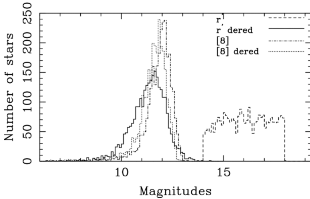
Figure 9. from Iphas A-Type Stars with Mid-Infrared Excesses in Spitzer Surveys HALES ET AL. 2009 ApJ 695 75 doi:10.1088/0004-637X/695/1/75 https://dx.doi.org/10.1088/0004-637X/695/1/75 © 2009. The American Astronomical Society. All rights reserved.
