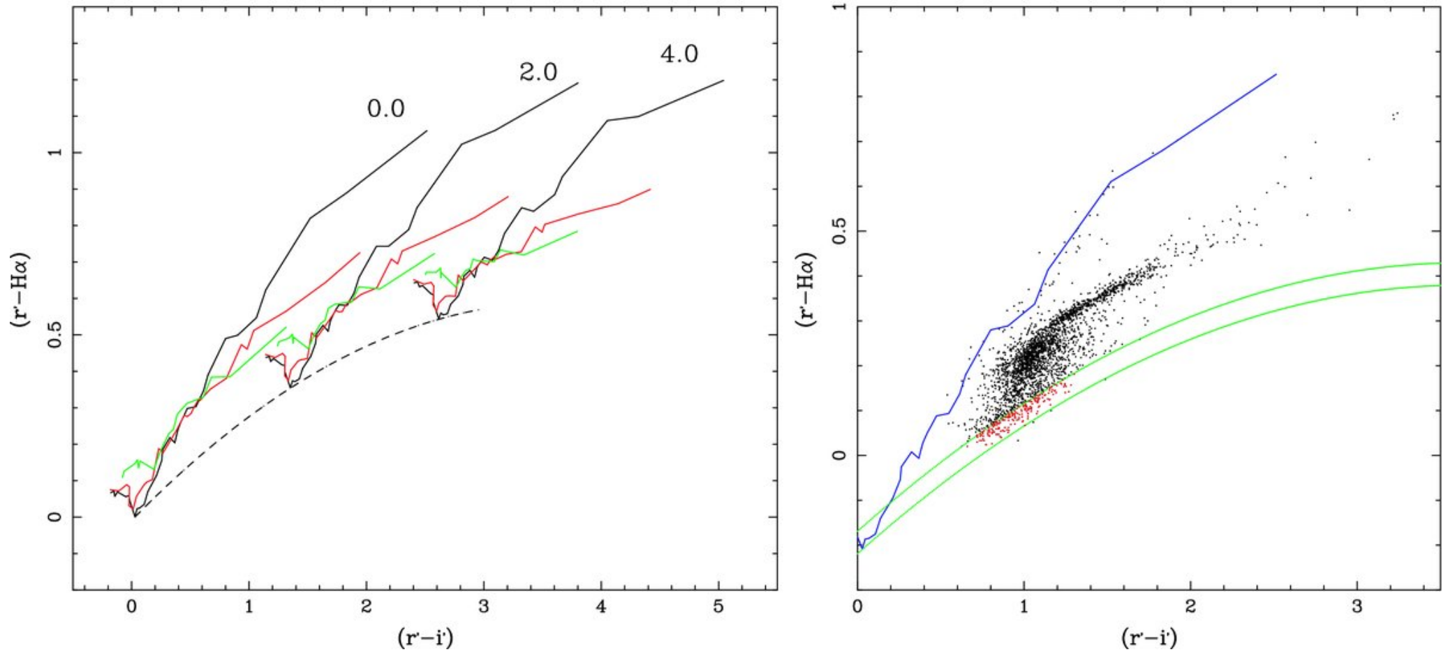
Figure 1. from Iphas A-Type Stars with Mid-Infrared Excesses in Spitzer Surveys HALES ET AL. 2009 ApJ 695 75 doi:10.1088/0004-637X/695/1/75 https://dx.doi.org/10.1088/0004-637X/695/1/75 © 2009. The American Astronomical Society. All rights reserved.
