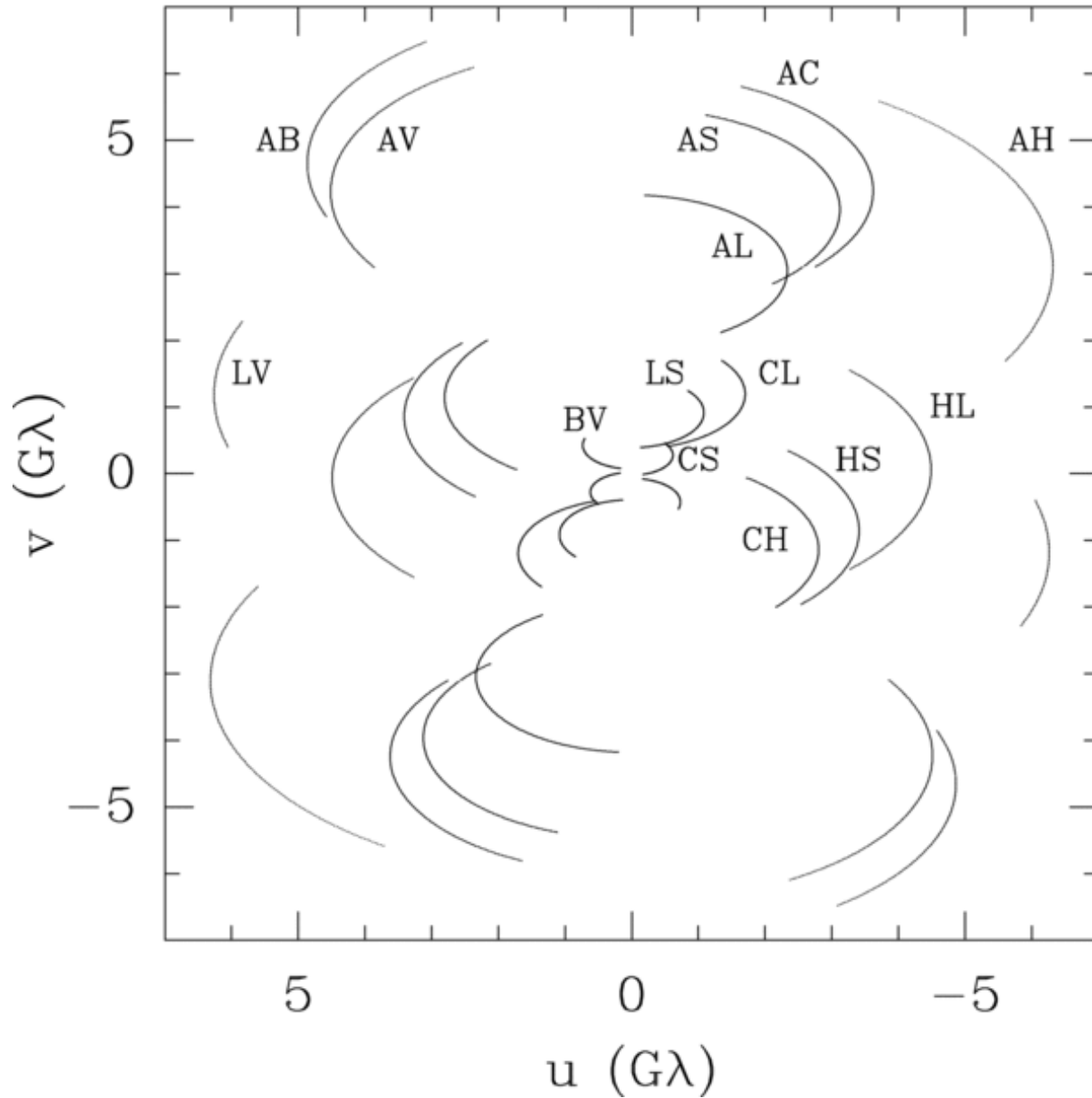
Figure 3. from Detecting Flaring Structures in Sagittarius A* with High-Frequency VLBI DOELEMAN ET AL. 2009 ApJ 695 59 doi:10.1088/0004-637X/695/1/59 https://dx.doi.org/10.1088/0004-637X/695/1/59 © 2009. The American Astronomical Society. All rights reserved.
