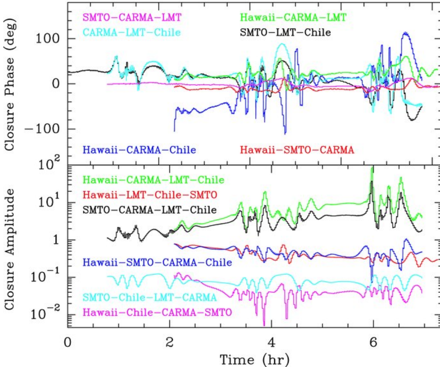
Figure 10. from Detecting Flaring Structures in Sagittarius A* with High-Frequency VLBI DOELEMAN ET AL. 2009 ApJ 695 59 doi:10.1088/0004-637X/695/1/59 https://dx.doi.org/10.1088/0004-637X/695/1/59 © 2009. The American Astronomical Society. All rights reserved.
