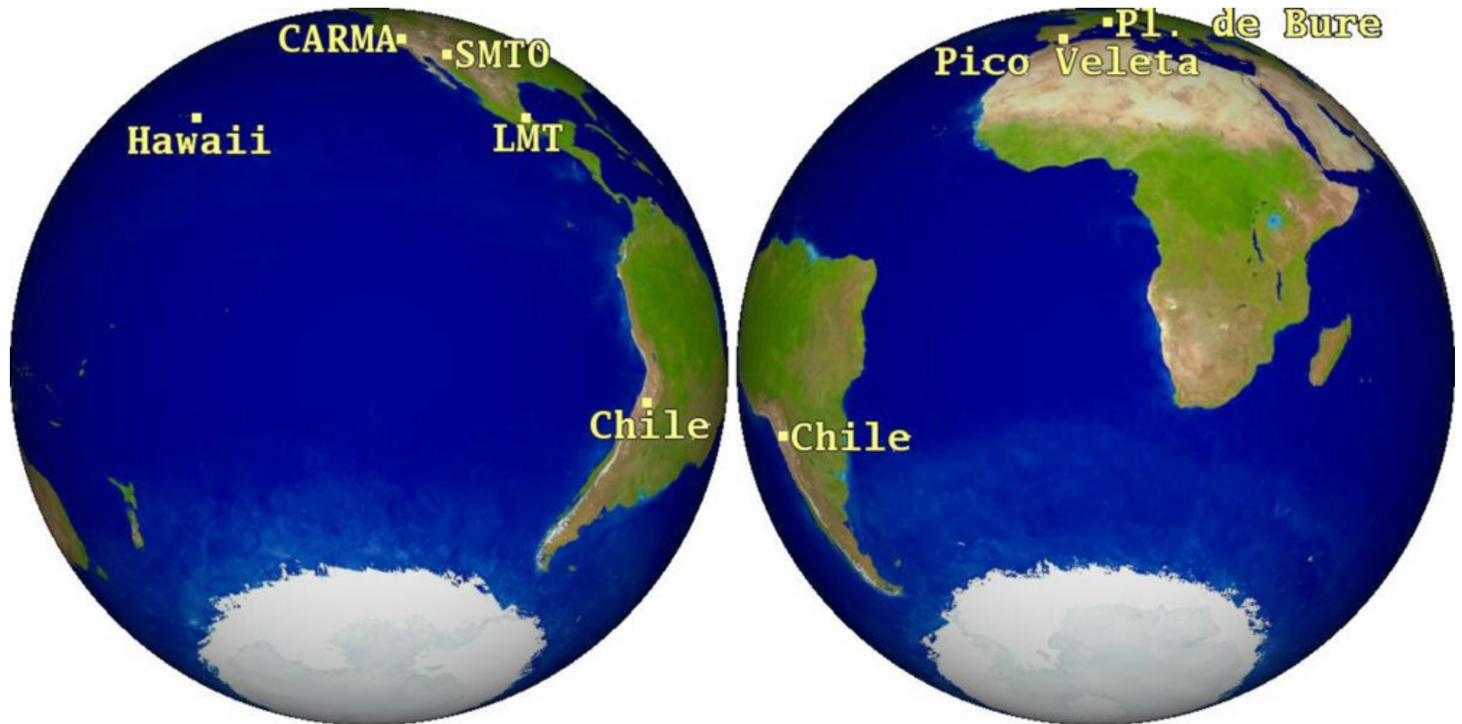
Figure 1. from Detecting Flaring Structures in Sagittarius A* with High-Frequency VLBI DOELEMEN ET AL. 2009 ApJ 695 59 doi:10.1088/0004-637X/695/1/59 https://dx.doi.org/10.1088/0004-637X/695/1/59 © 2009. The American Astronomical Society. All rights reserved.
