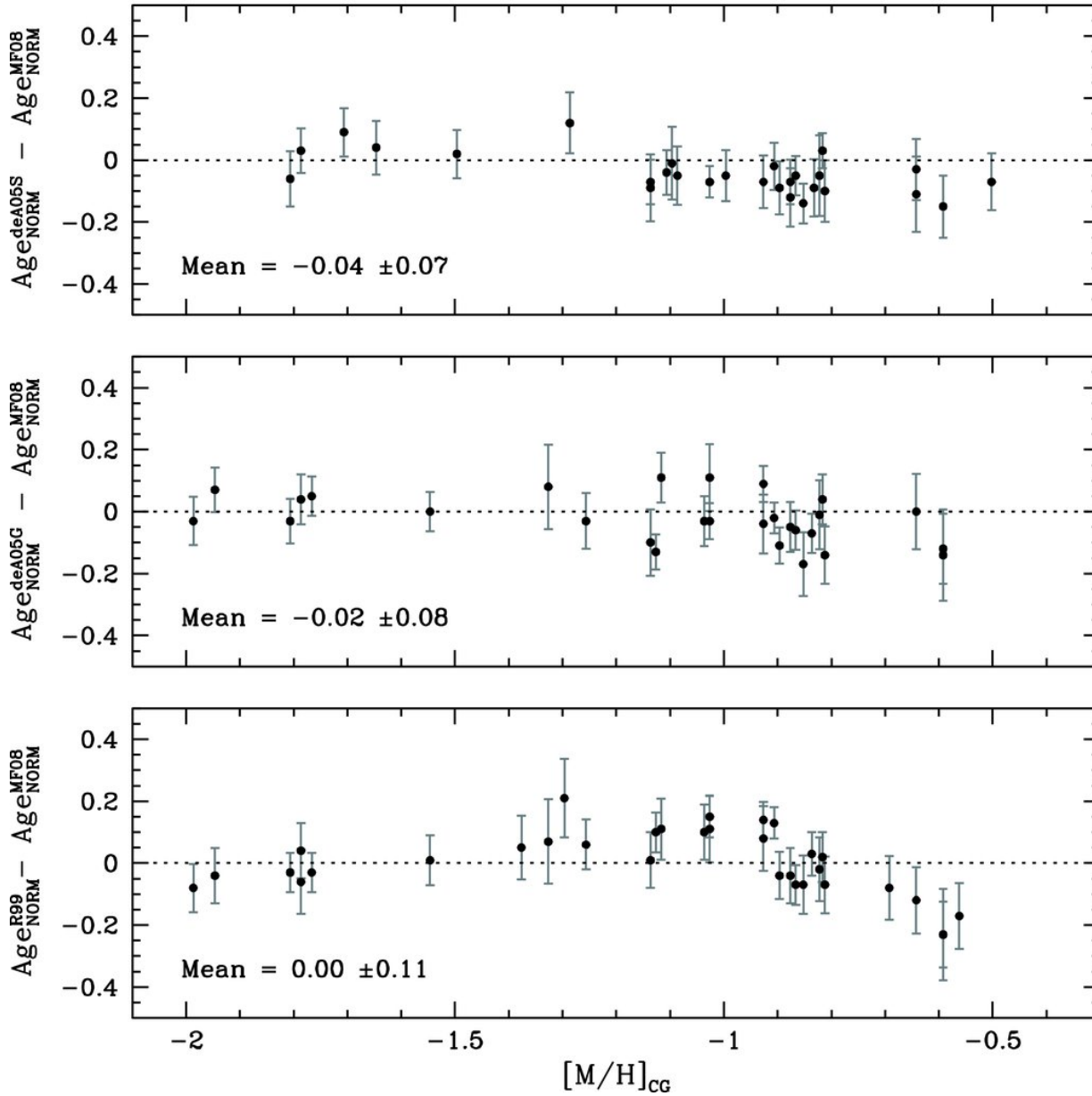
Figure 9. from The ACS Survey of Galactic Globular Clusters. VII. Relative Ages MARÍN-FRANCH ET AL. 2009 ApJ 694 1498 doi:10.1088/0004-637X/694/2/1498 https://dx.doi.org/10.1088/0004-637X/694/2/1498
