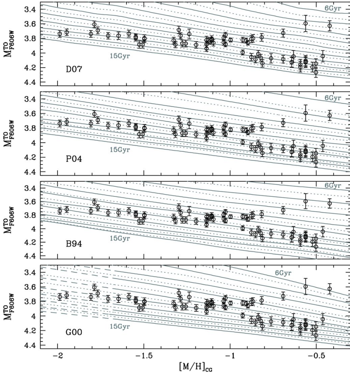
Figure 7. from The ACS Survey of Galactic Globular Clusters. VII. Relative Ages MARÍN-FRANCH ET AL. 2009 ApJ 694 1498 doi:10.1088/0004-637X/694/2/1498 https://dx.doi.org/10.1088/0004-637X/694/2/1498
