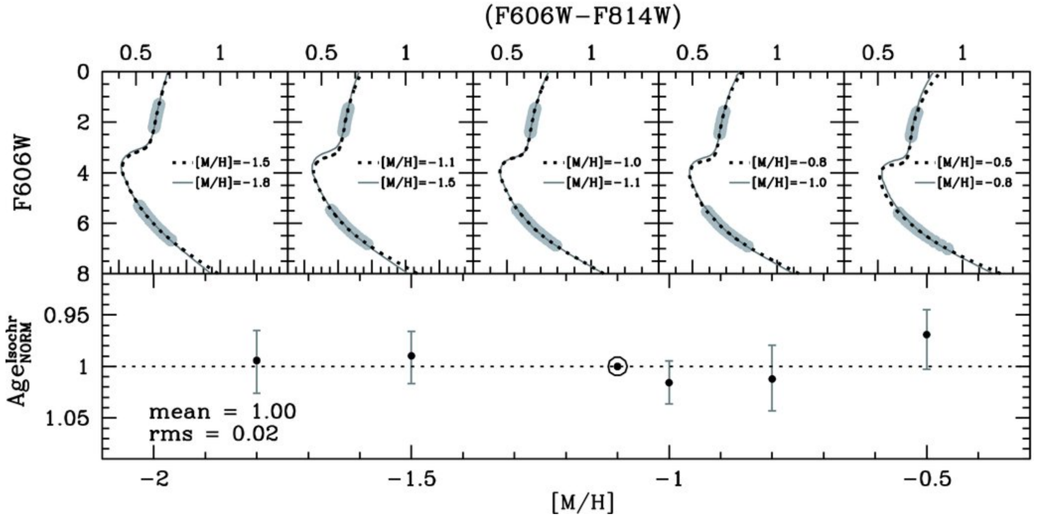
Figure 6. from The ACS Survey of Galactic Globular Clusters. VII. Relative Ages MARÍN-FRANCH ET AL. 2009 ApJ 694 1498 doi:10.1088/0004-637X/694/2/1498 https://dx.doi.org/10.1088/0004-637X/694/2/1498 © 2009. The American Astronomical Society. All rights reserved.
