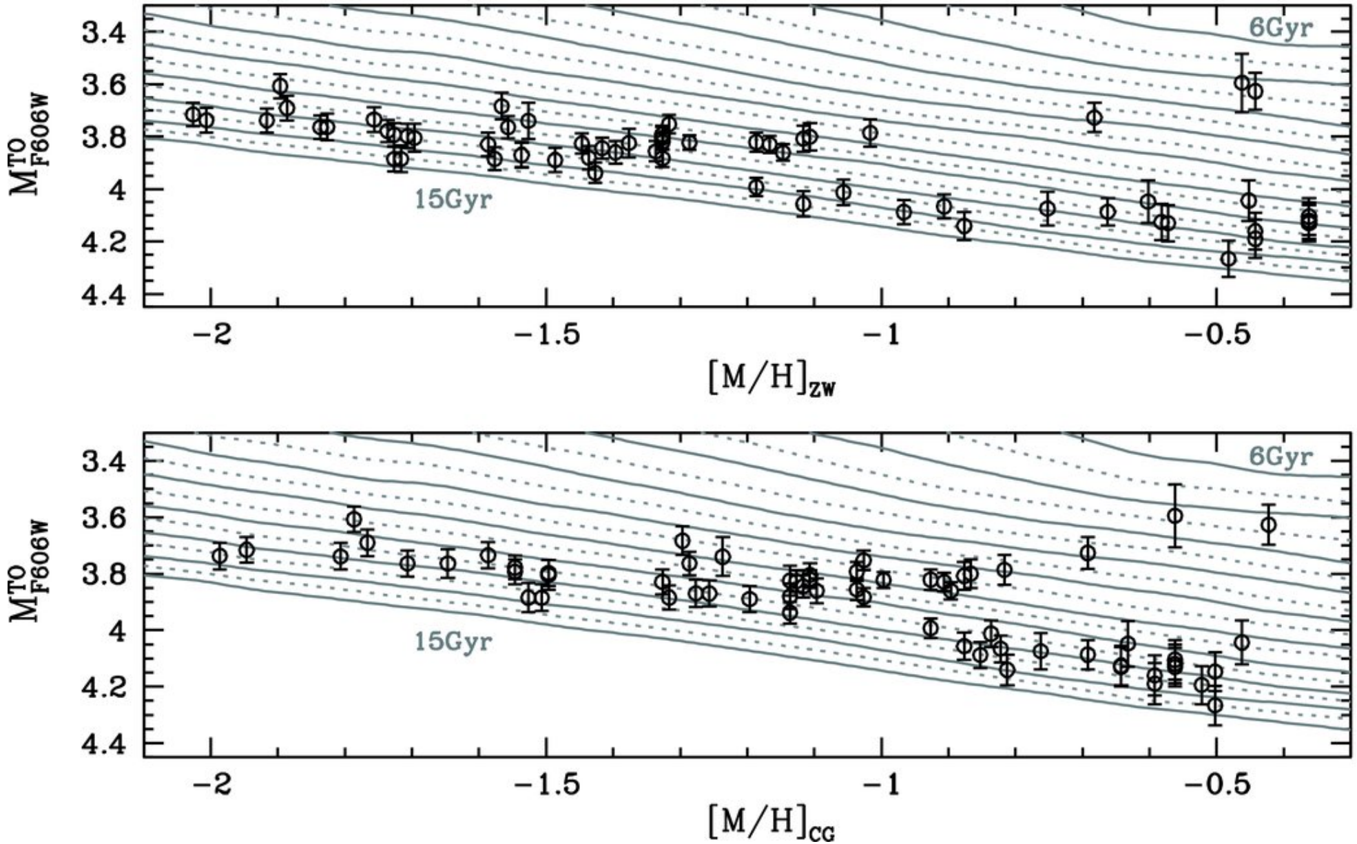
Figure 5. from The ACS Survey of Galactic Globular Clusters. VII. Relative Ages MARÍN-FRANCH ET AL. 2009 ApJ 694 1498 doi:10.1088/0004-637X/694/2/1498 https://dx.doi.org/10.1088/0004-637X/694/2/1498 © 2009. The American Astronomical Society. All rights reserved.
