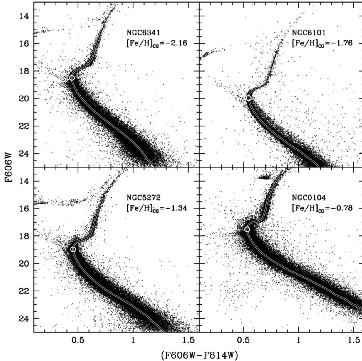
Figure 2. from The ACS Survey of Galactic Globular Clusters. VII. Relative Ages MARÍN-FRANCH ET AL. 2009 ApJ 694 1498 doi:10.1088/0004-637X/694/2/1498 https://dx.doi.org/10.1088/0004-637X/694/2/1498 © 2009. The American Astronomical Society. All rights reserved.
