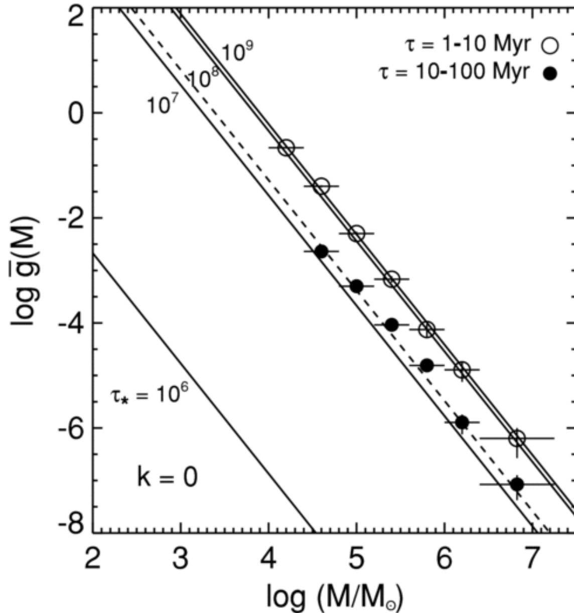
Figure 8. from New Tests for Disruption Mechanisms of Star Clusters: Methods and Application to the Antennae Galaxies FALL, CHANDAR, & WHITMORE 2009 ApJ 704 453 doi:10.1088/0004-637X/704/1/453 https://dx.doi.org/10.1088/0004-637X/704/1/453 © 2009. The American Astronomical Society. All rights reserved.
