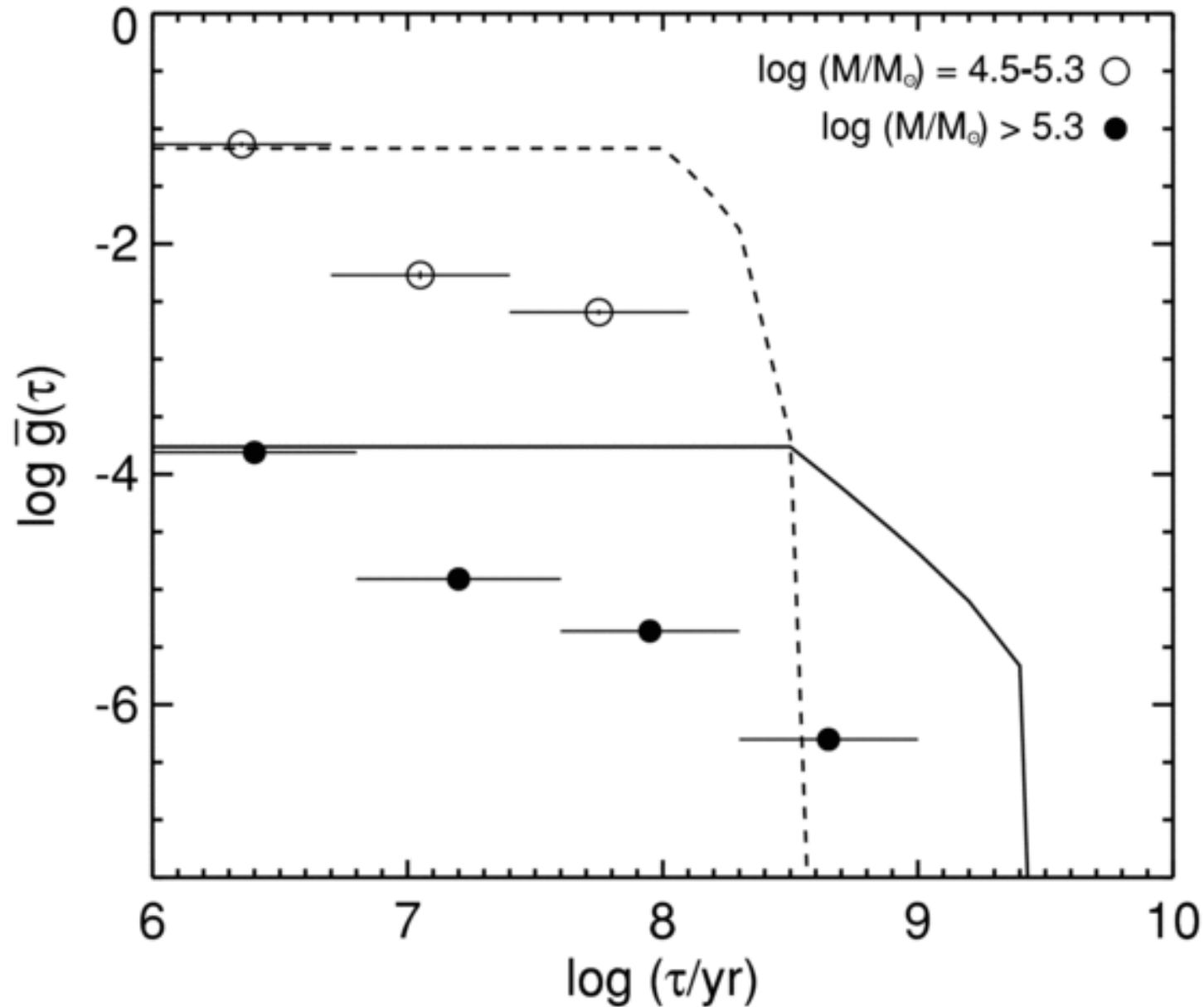
Figure 7. from New Tests for Disruption Mechanisms of Star Clusters: Methods and Application to the Antennae Galaxies FALL, CHANDAR, & WHITMORE 2009 ApJ 704 453 doi:10.1088/0004-637X/704/1/453 https://dx.doi.org/10.1088/0004-637X/704/1/453 © 2009. The American Astronomical Society. All rights reserved.
