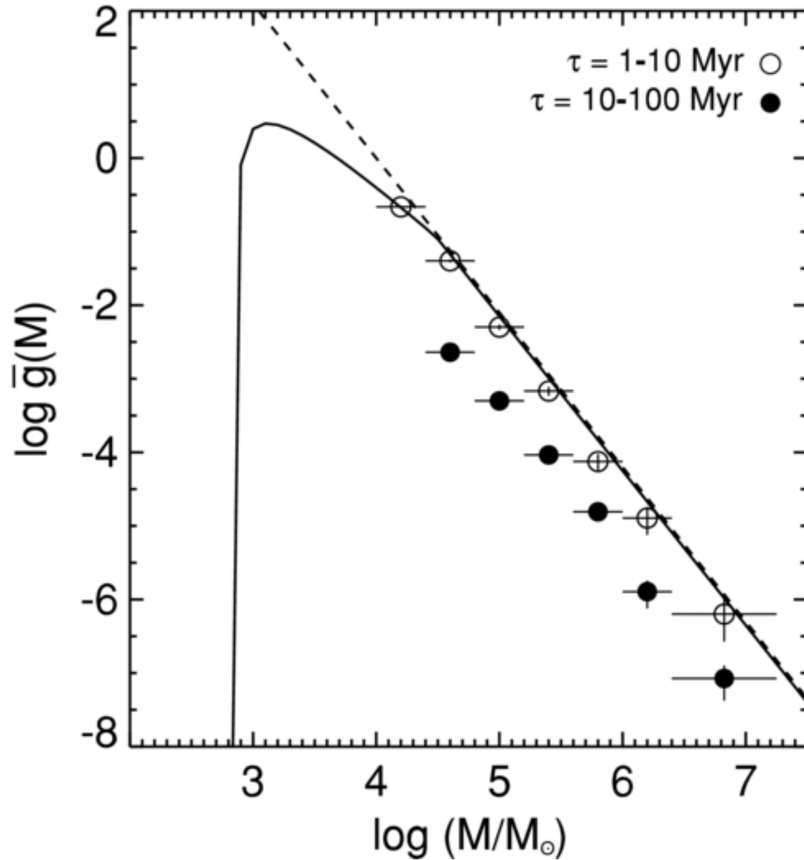
Figure 6. from New Tests for Disruption Mechanisms of Star Clusters: Methods and Application to the Antennae Galaxies FALL, CHANDAR, & WHITMORE 2009 ApJ 704 453 doi:10.1088/0004-637X/704/1/453 https://dx.doi.org/10.1088/0004-637X/704/1/453 © 2009. The American Astronomical Society. All rights reserved.
