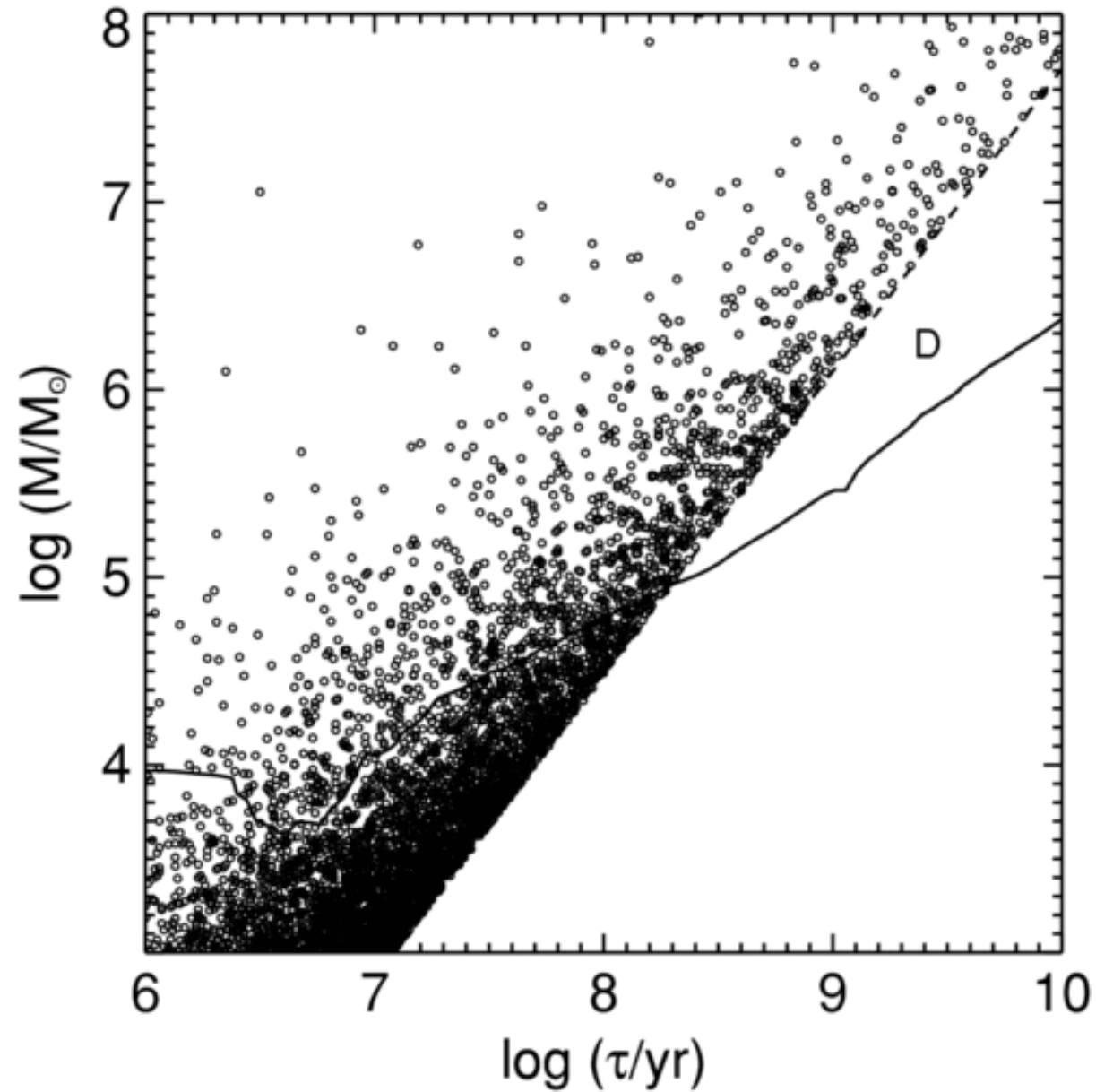
Figure 5. from New Tests for Disruption Mechanisms of Star Clusters: Methods and Application to the Antennae Galaxies FALL, CHANDAR, & WHITMORE 2009 ApJ 704 453 doi:10.1088/0004-637X/704/1/453 https://dx.doi.org/10.1088/0004-637X/704/1/453 © 2009. The American Astronomical Society. All rights reserved.
