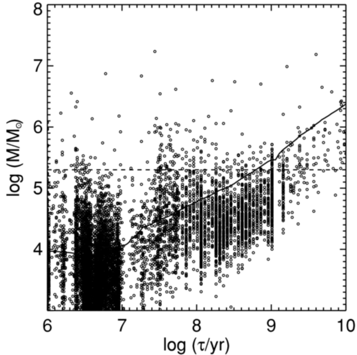
Figure 2. from New Tests for Disruption Mechanisms of Star Clusters: Methods and Application to the Antennae Galaxies FALL, CHANDAR, & WHITMORE 2009 ApJ 704 453 doi:10.1088/0004-637X/704/1/453 https://dx.doi.org/10.1088/0004-637X/704/1/453 © 2009. The American Astronomical Society. All rights reserved.
