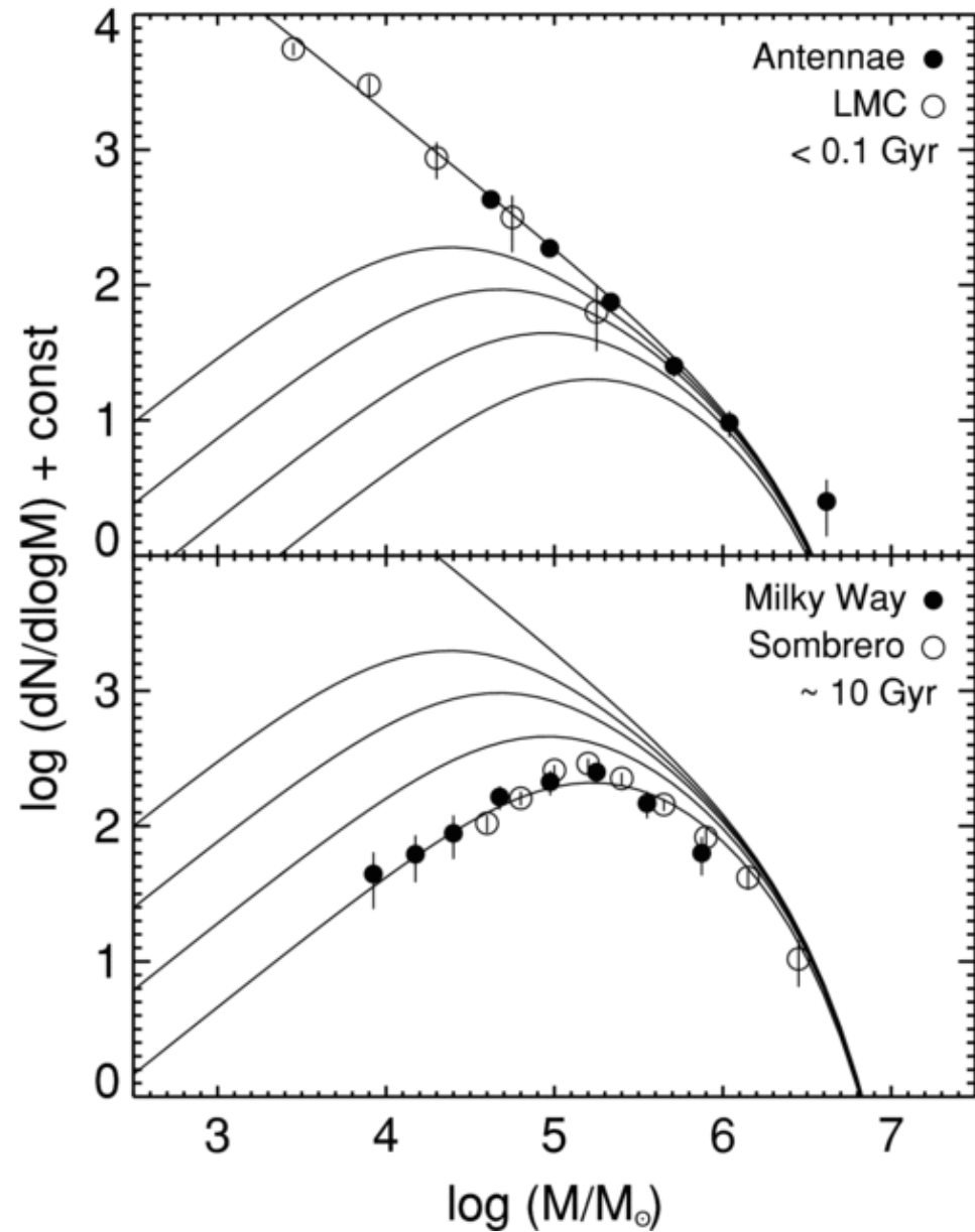
Figure 14. from New Tests for Disruption Mechanisms of Star Clusters: Methods and Application to the Antennae Galaxies FALL, CHANDAR, & WHITMORE 2009 ApJ 704 453 doi:10.1088/0004-637X/704/1/453 https://dx.doi.org/10.1088/0004-637X/704/1/453 © 2009. The American Astronomical Society. All rights reserved.
