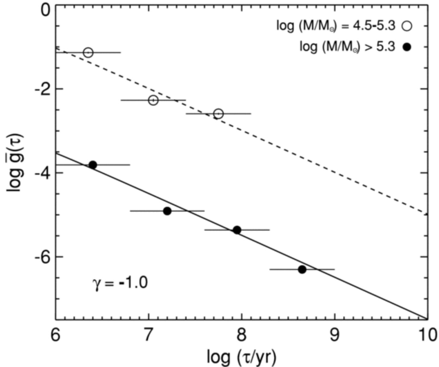
Figure 13. from New Tests for Disruption Mechanisms of Star Clusters: Methods and Application to the Antennae Galaxies FALL, CHANDAR, & WHITMORE 2009 ApJ 704 453 doi:10.1088/0004-637X/704/1/453 https://dx.doi.org/10.1088/0004-637X/704/1/453 © 2009. The American Astronomical Society. All rights reserved.
