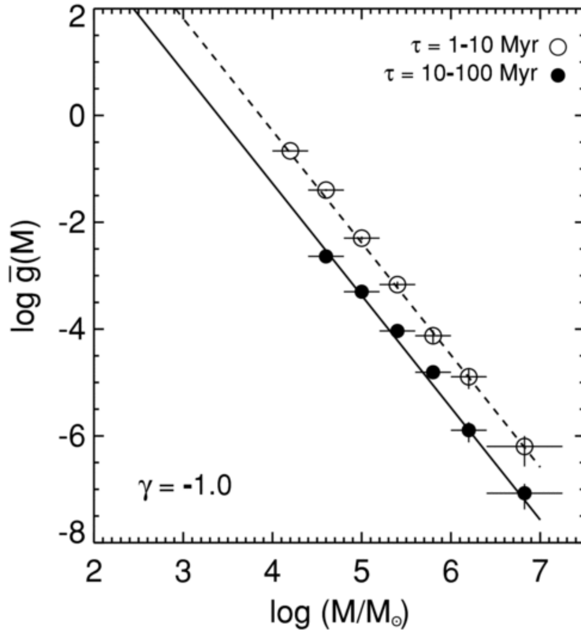
Figure 12. from New Tests for Disruption Mechanisms of Star Clusters: Methods and Application to the Antennae Galaxies FALL, CHANDAR, & WHITMORE 2009 ApJ 704 453 doi:10.1088/0004-637X/704/1/453 https://dx.doi.org/10.1088/0004-637X/704/1/453 © 2009. The American Astronomical Society. All rights reserved.
