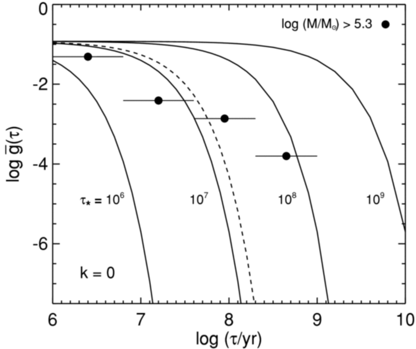
Figure 11. from New Tests for Disruption Mechanisms of Star Clusters: Methods and Application to the Antennae Galaxies FALL, CHANDAR, & WHITMORE 2009 ApJ 704 453 doi:10.1088/0004-637X/704/1/453 https://dx.doi.org/10.1088/0004-637X/704/1/453 © 2009. The American Astronomical Society. All rights reserved.
