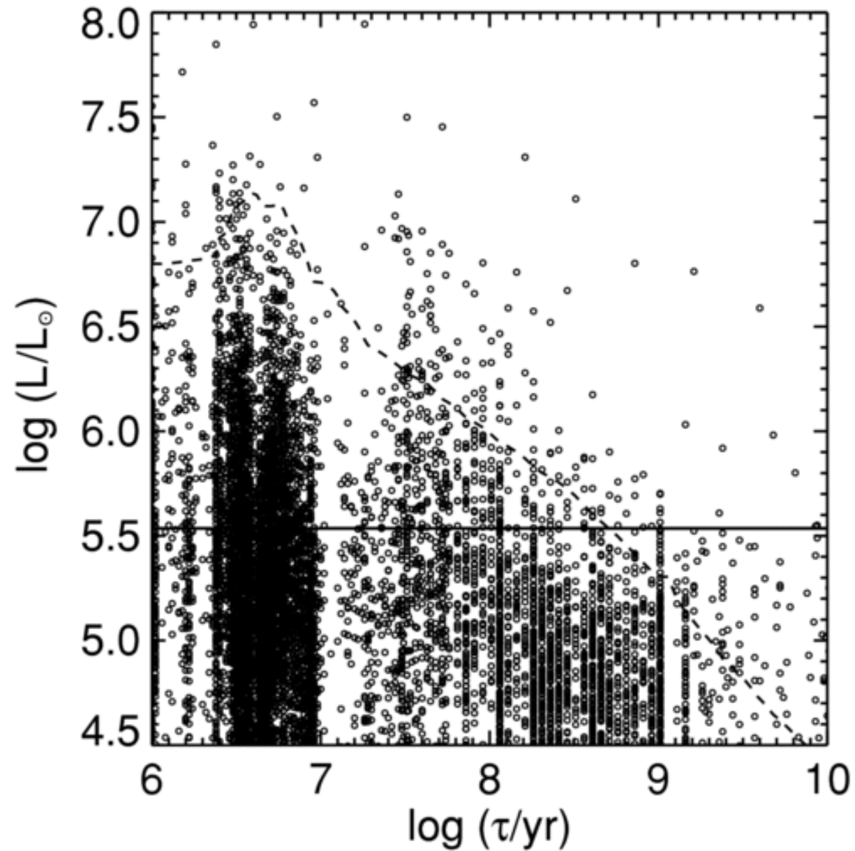
Figure 1. from New Tests for Disruption Mechanisms of Star Clusters: Methods and Application to the Antennae Galaxies FALL, CHANDAR, & WHITMORE 2009 ApJ 704 453 doi:10.1088/0004-637X/704/1/453 https://dx.doi.org/10.1088/0004-637X/704/1/453 © 2009. The American Astronomical Society. All rights reserved.
