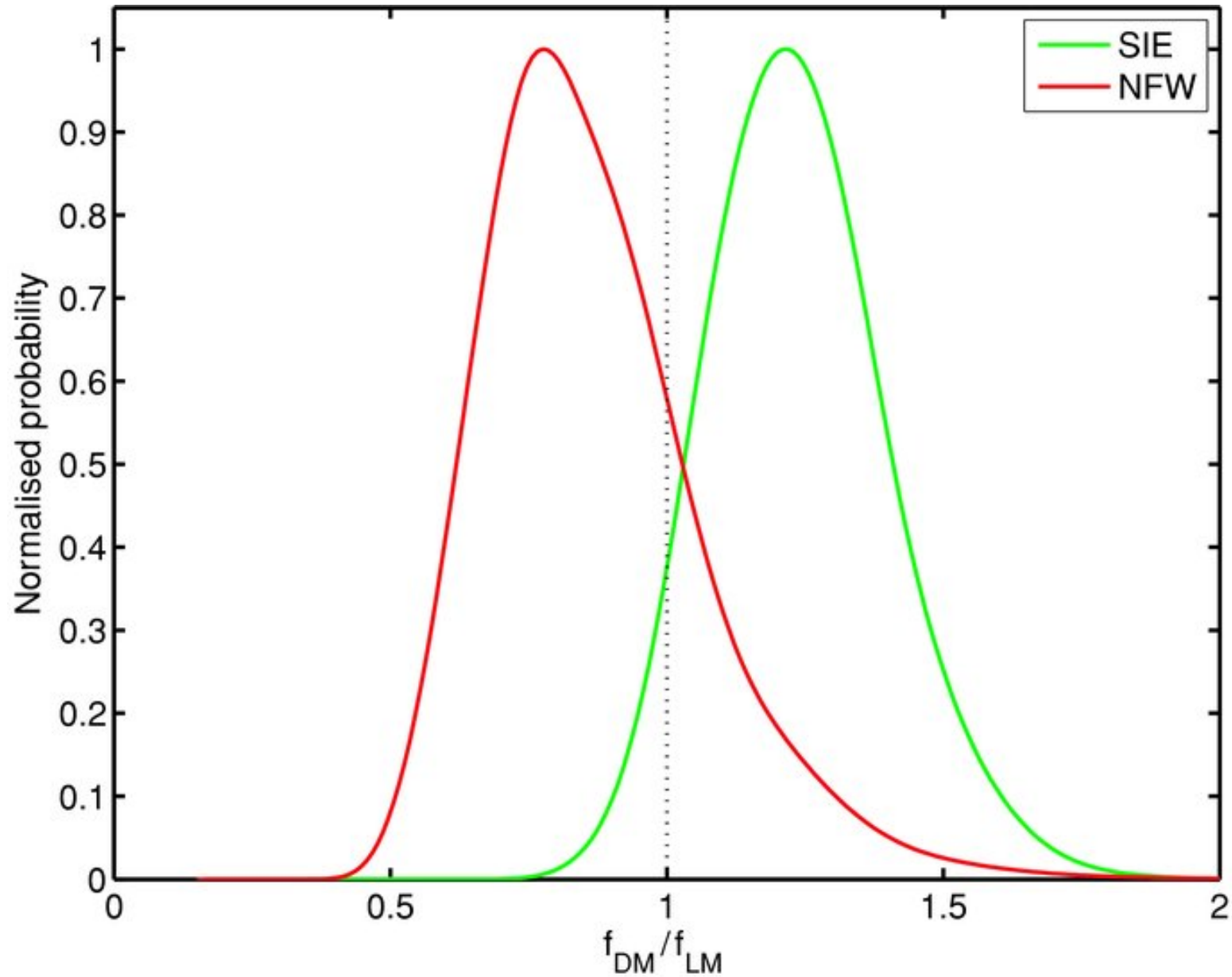
Figure 5. from A Detection of Dark Matter Halo Ellipticity using Galaxy Cluster Lensing in the SDSS EVANS & BRIDLE 2009 ApJ 695 1446 doi:10.1088/0004-637X/695/2/1446 https://dx.doi.org/10.1088/0004-637X/695/2/1446 © 2009. The American Astronomical Society. All rights reserved.
