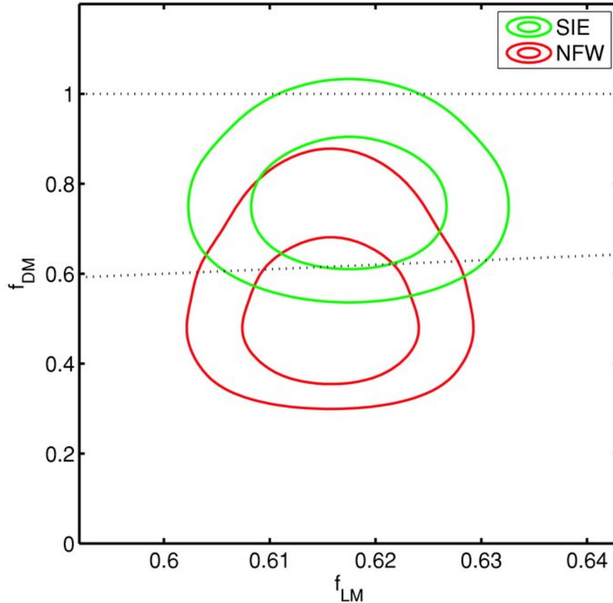
Figure 4. from A Detection of Dark Matter Halo Ellipticity using Galaxy Cluster Lensing in the SDSS EVANS & BRIDLE 2009 ApJ 695 1446 doi:10.1088/0004-637X/695/2/1446 https://dx.doi.org/10.1088/0004-637X/695/2/1446 © 2009. The American Astronomical Society. All rights reserved.
